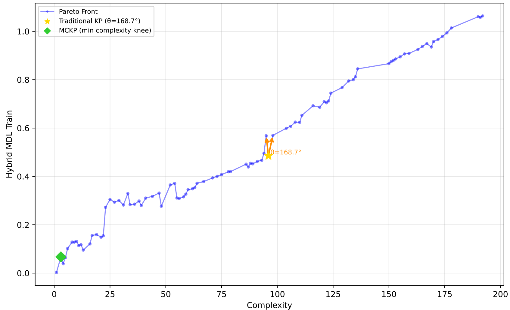
542_pollution - Run 5 - MVP - Hybrid MDL Train \lambda_1=1.00, \lambda_2=0.10, \lambda_3=0.00 | Difficulty: 0.59 | Method: mckp
