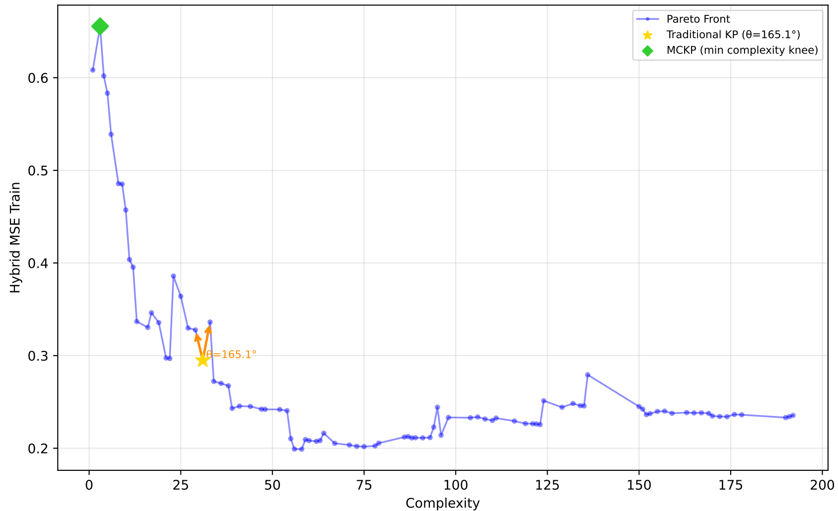
542_pollution - Run 5 - MVP - Hybrid MSE Train \lambda_1=1.00, \lambda_2=0.10, \lambda_3=0.00 | Difficulty: 0.59 | Method: mckp
