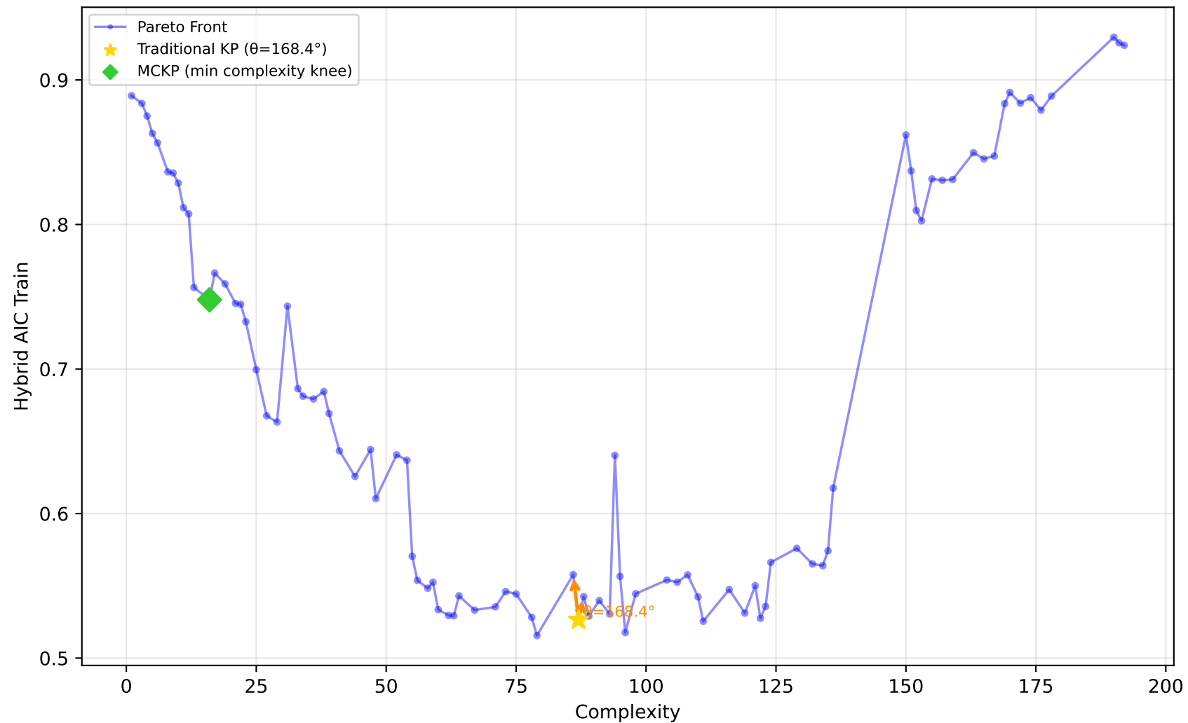
542_pollution - Run 5 - SVP - Hybrid AIC Train \lambda_1=0.00, \lambda_2=0.00, \lambda_3=0.20 | Difficulty: 0.59 | Method: mckp
