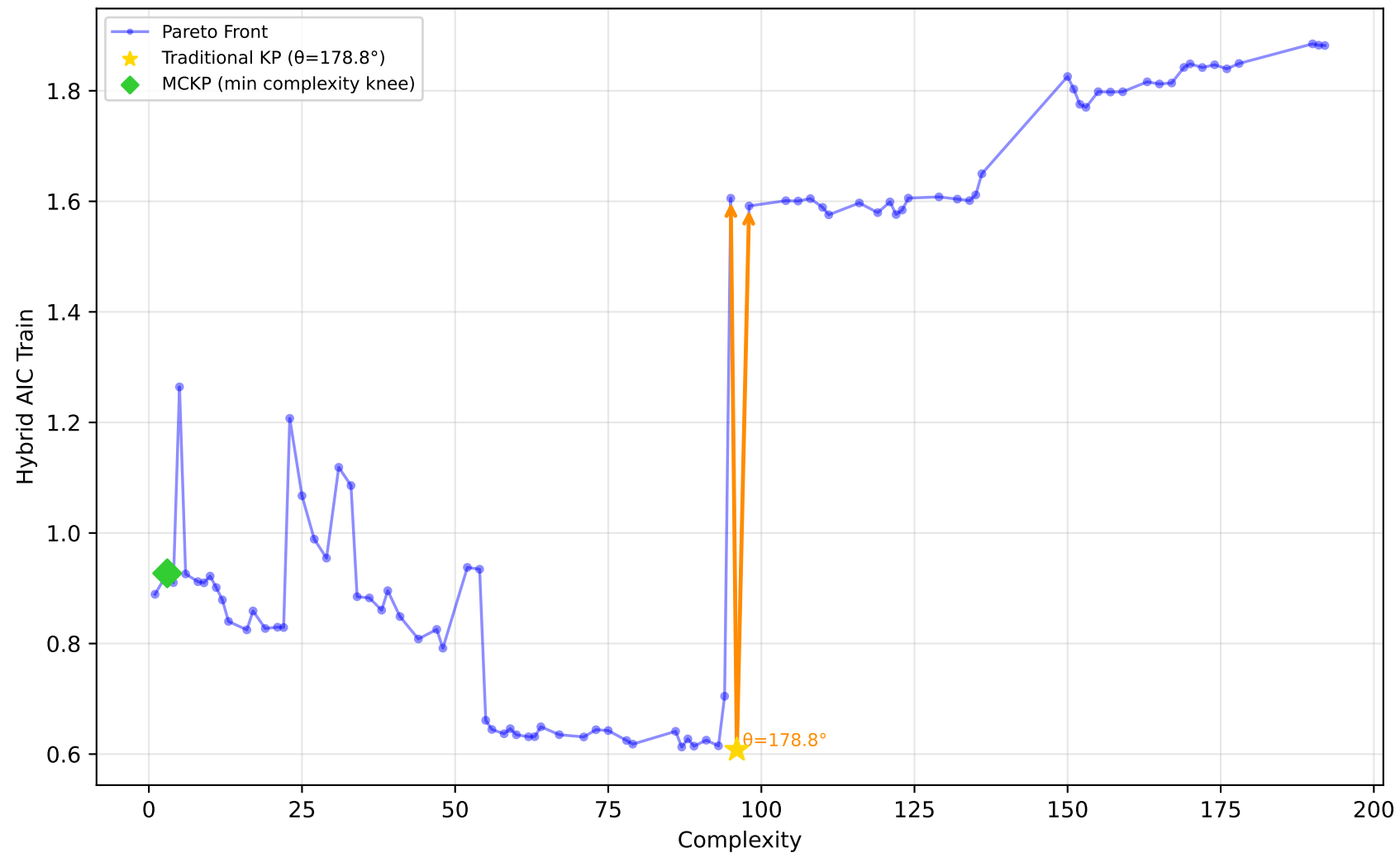
542_pollution - Run 5 - SVP - Hybrid AIC Train \lambda_1=0.70, \lambda_2=1.00, \lambda_3=0.10 | Difficulty: 0.59 | Method: mckp
