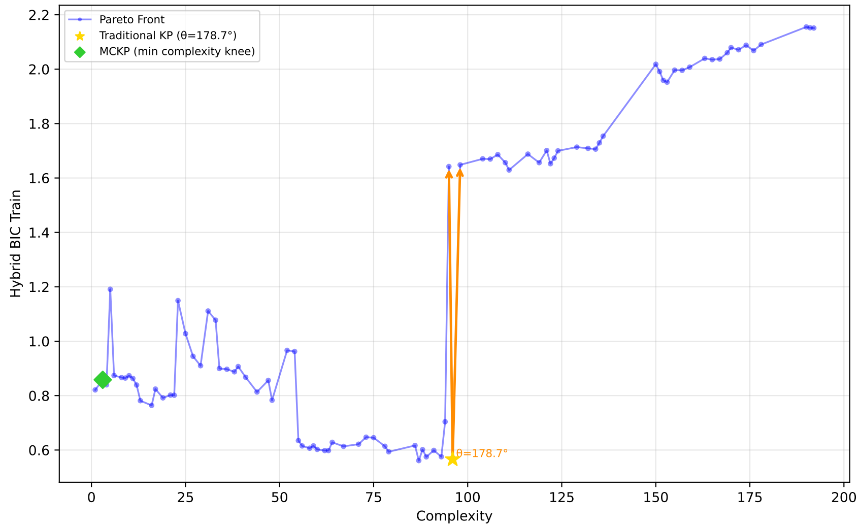
542_pollution - Run 5 - SVP - Hybrid BIC Train \lambda_1=0.70, \lambda_2=1.00, \lambda_3=0.10 | Difficulty: 0.59 | Method: mckp
