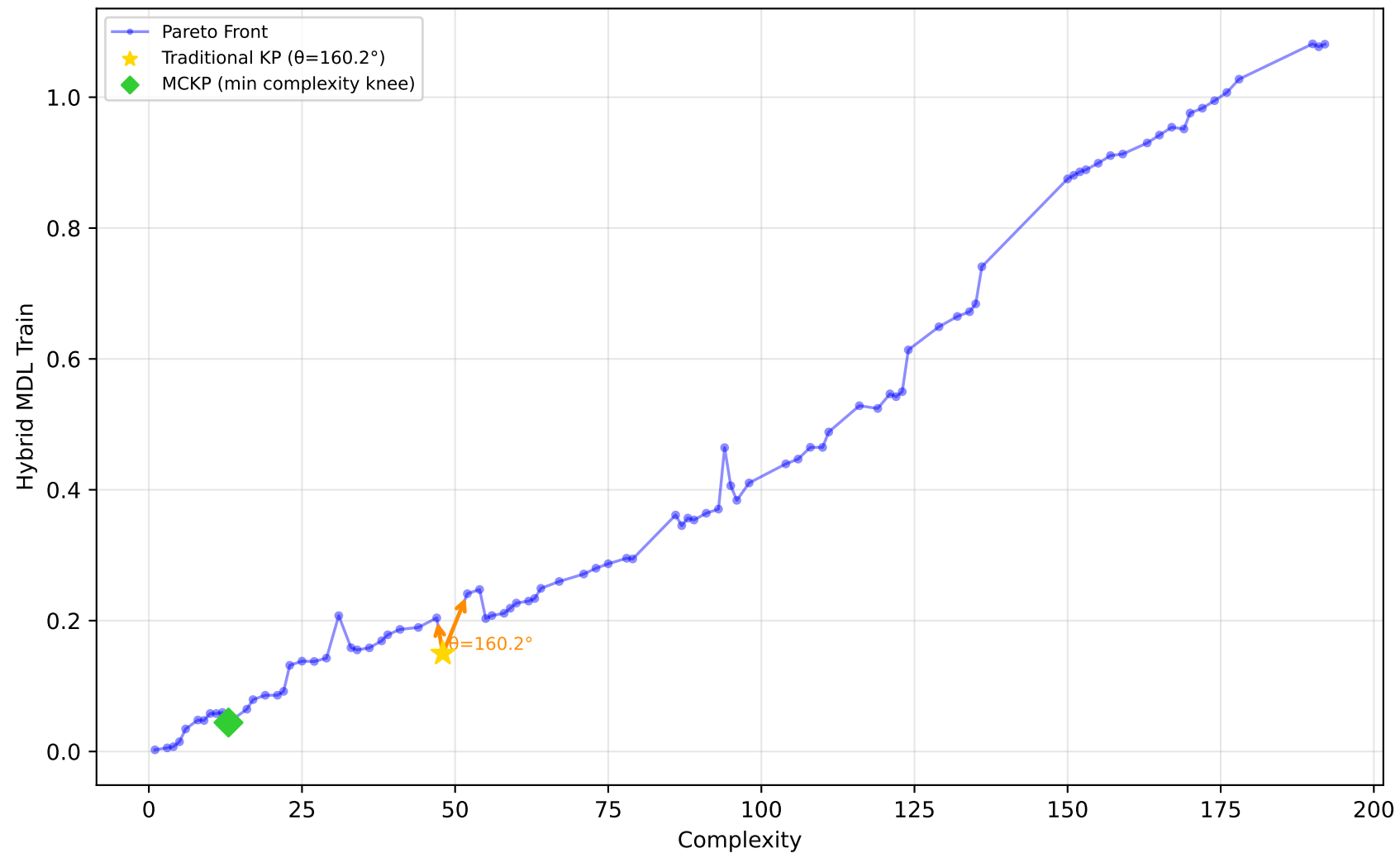
542_pollution - Run 5 - SVP - Hybrid MDL Train \lambda_1=0.00, \lambda_2=0.00, \lambda_3=0.20 | Difficulty: 0.59 | Method: mckp
