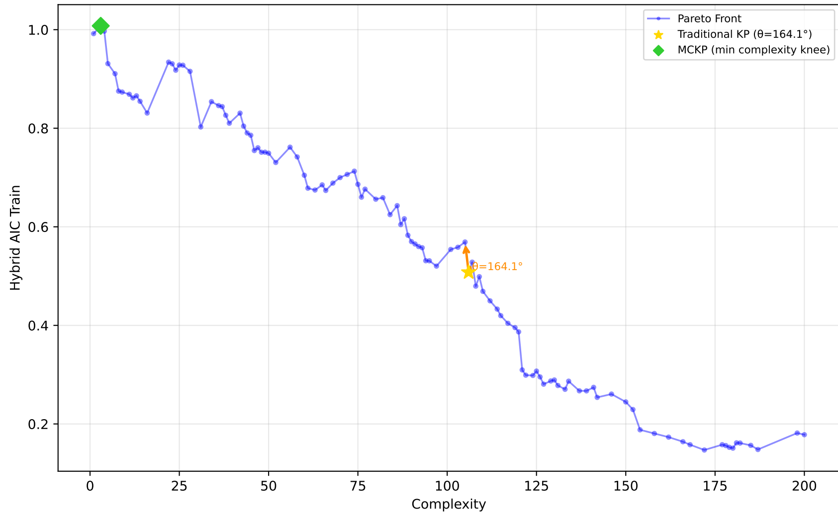
542_pollution - Run 6 - MVP - Hybrid AIC Train \lambda_1=0.40, \lambda_2=0.10, \lambda_3=0.00 | Difficulty: 0.29 | Method: mckp
