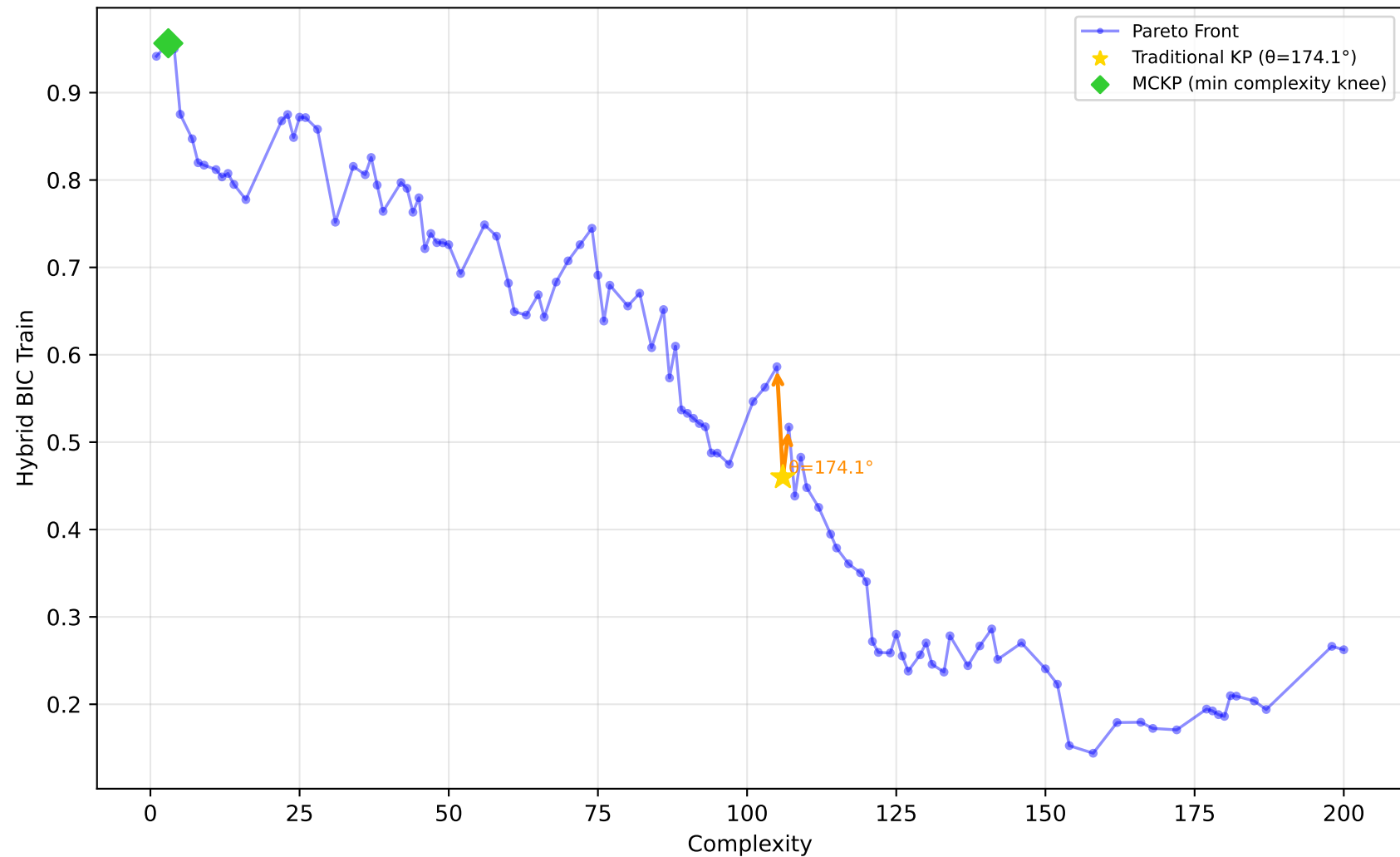
542_pollution - Run 6 - MVP - Hybrid BIC Train \lambda_1=0.40, \lambda_2=0.10, \lambda_3=0.00 | Difficulty: 0.29 | Method: mckp
