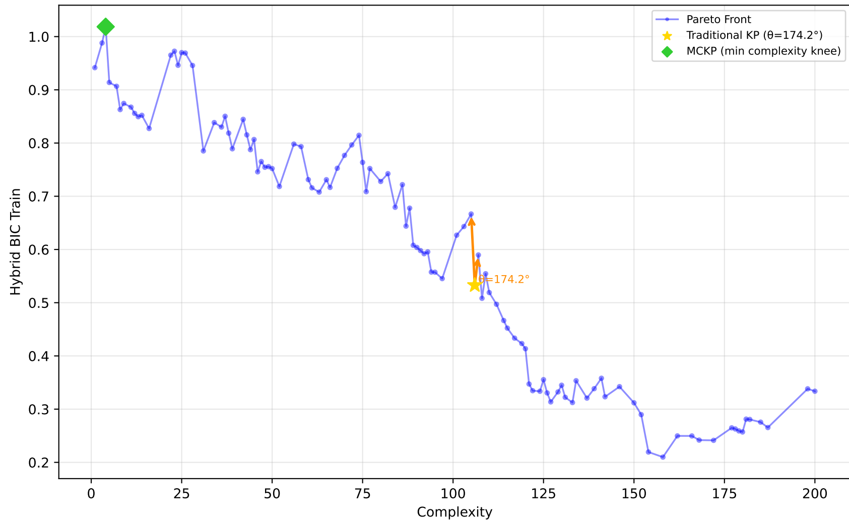
542_pollution - Run 6 - MVP - Hybrid BIC Train \lambda_1=1.00, \lambda_2=0.10, \lambda_3=0.00 | Difficulty: 0.29 | Method: mckp
