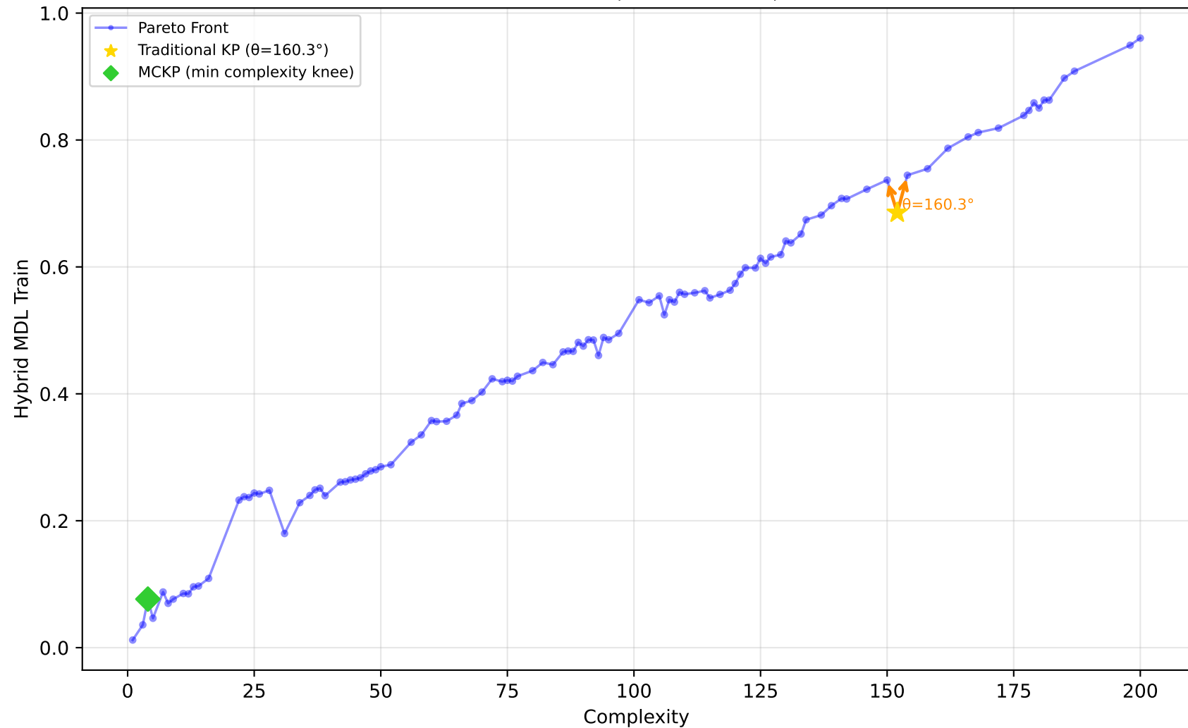
542_pollution - Run 6 - MVP - Hybrid MDL Train \lambda_1=0.40, \lambda_2=0.10, \lambda_3=0.00 | Difficulty: 0.29 | Method: mckp
