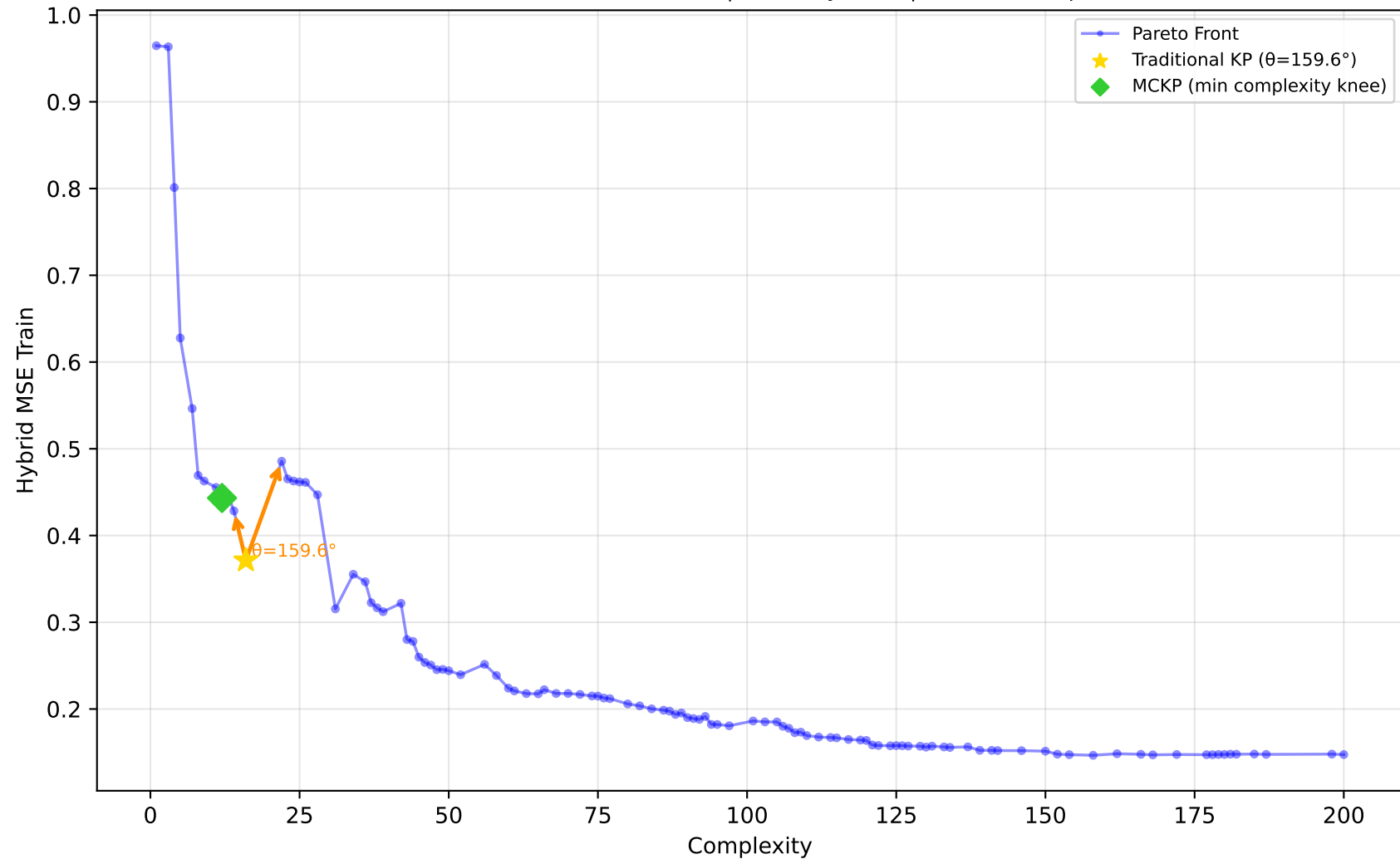
542_pollution - Run 6 - MVP - Hybrid MSE Train \lambda_1=0.40, \lambda_2=0.10, \lambda_3=0.00 | Difficulty: 0.29 | Method: mckp
