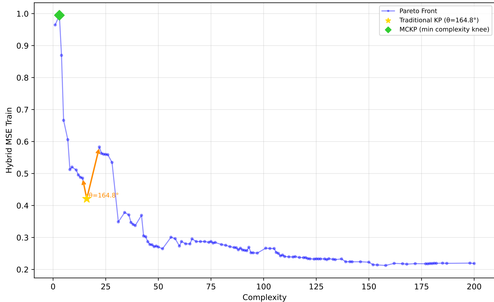
542_pollution - Run 6 - MVP - Hybrid MSE Train \lambda_1=1.00, \lambda_2=0.10, \lambda_3=0.00 | Difficulty: 0.29 | Method: mckp
