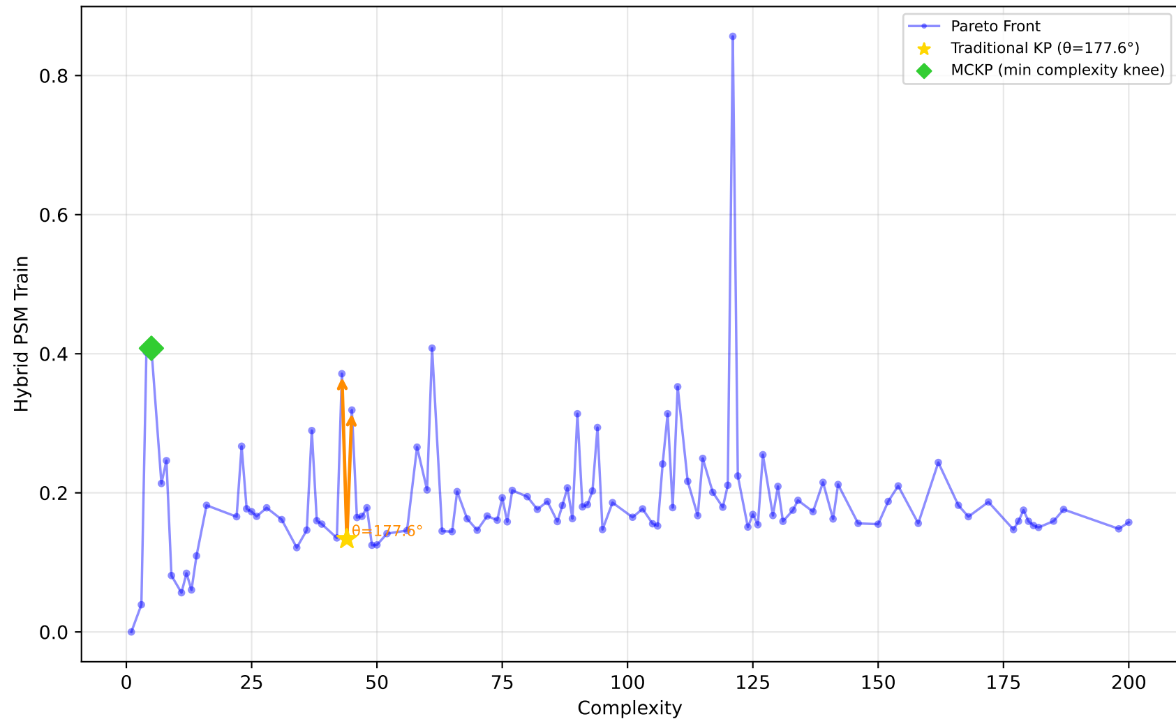
542_pollution - Run 6 - MVP - Hybrid PSM Train \lambda_1=0.40, \lambda_2=0.10, \lambda_3=0.00 | Difficulty: 0.29 | Method: mckp
