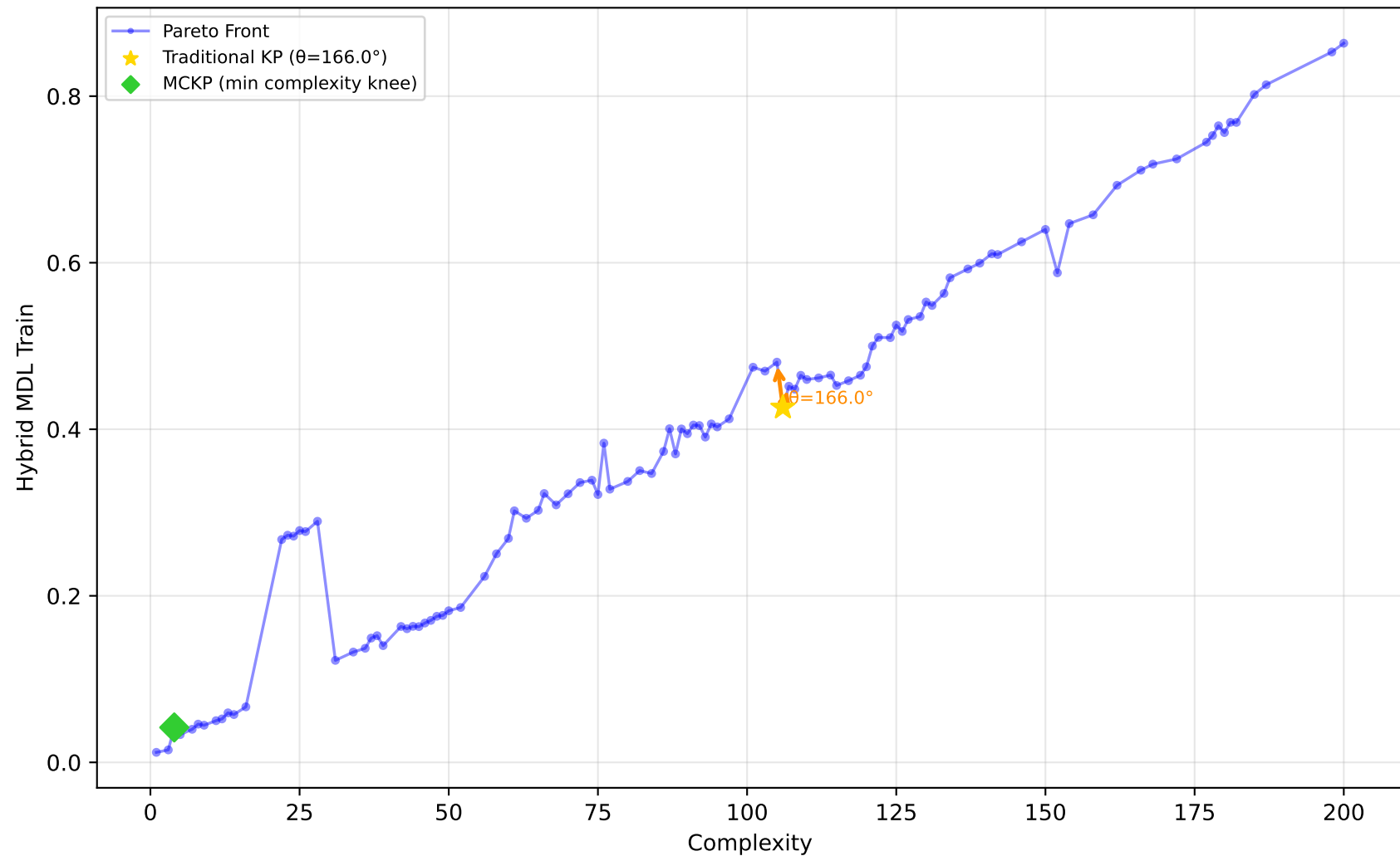
542_pollution - Run 6 - SVP - Hybrid MDL Train \lambda_1=0.00, \lambda_2=0.00, \lambda_3=0.20 | Difficulty: 0.29 | Method: mckp
