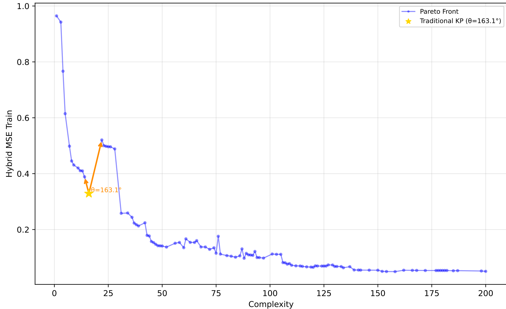
542_pollution - Run 6 - SVP - Hybrid MSE Train \lambda_1=0.00 , \lambda_2=0.00 , \lambda_3=0.20 | Difficulty: 0.29 | Method: mckp
