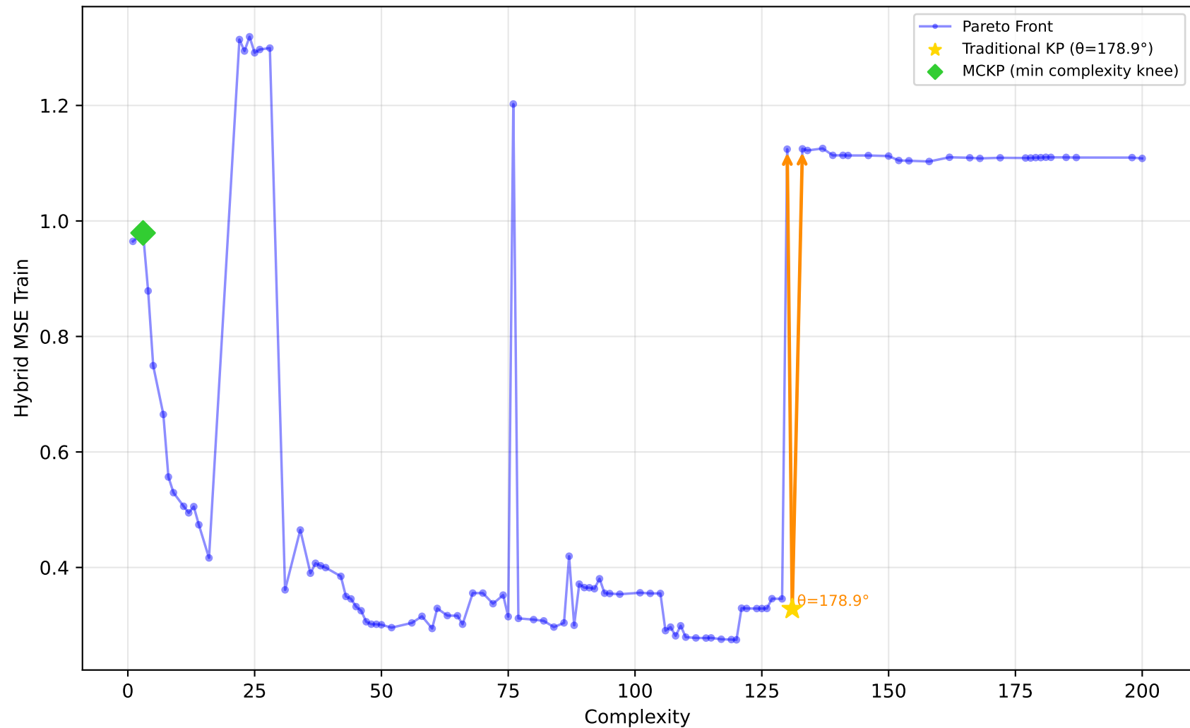
542_pollution - Run 6 - SVP - Hybrid MSE Train \lambda_1=0.70, \lambda_2=1.00, \lambda_3=0.10 | Difficulty: 0.29 | Method: mckp
