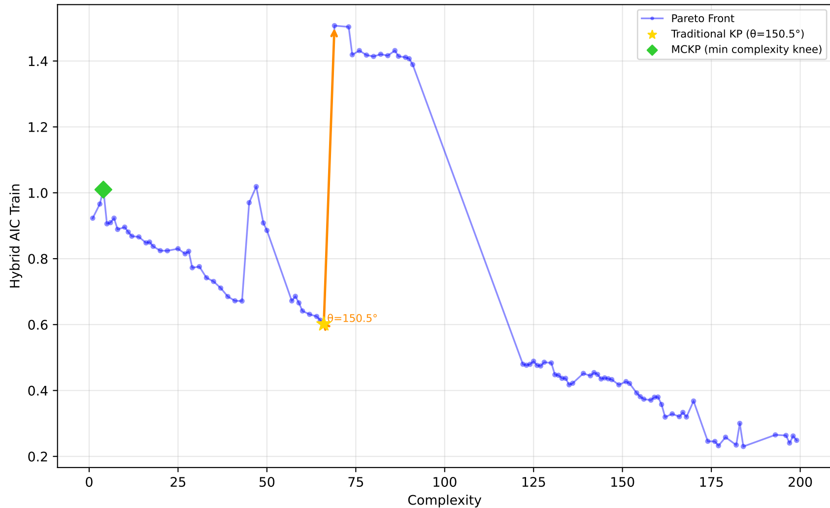
542_pollution - Run 7 - MVP - Hybrid AIC Train \lambda_1=1.00, \lambda_2=0.10, \lambda_3=0.00 | Difficulty: 1.00 | Method: hmr
