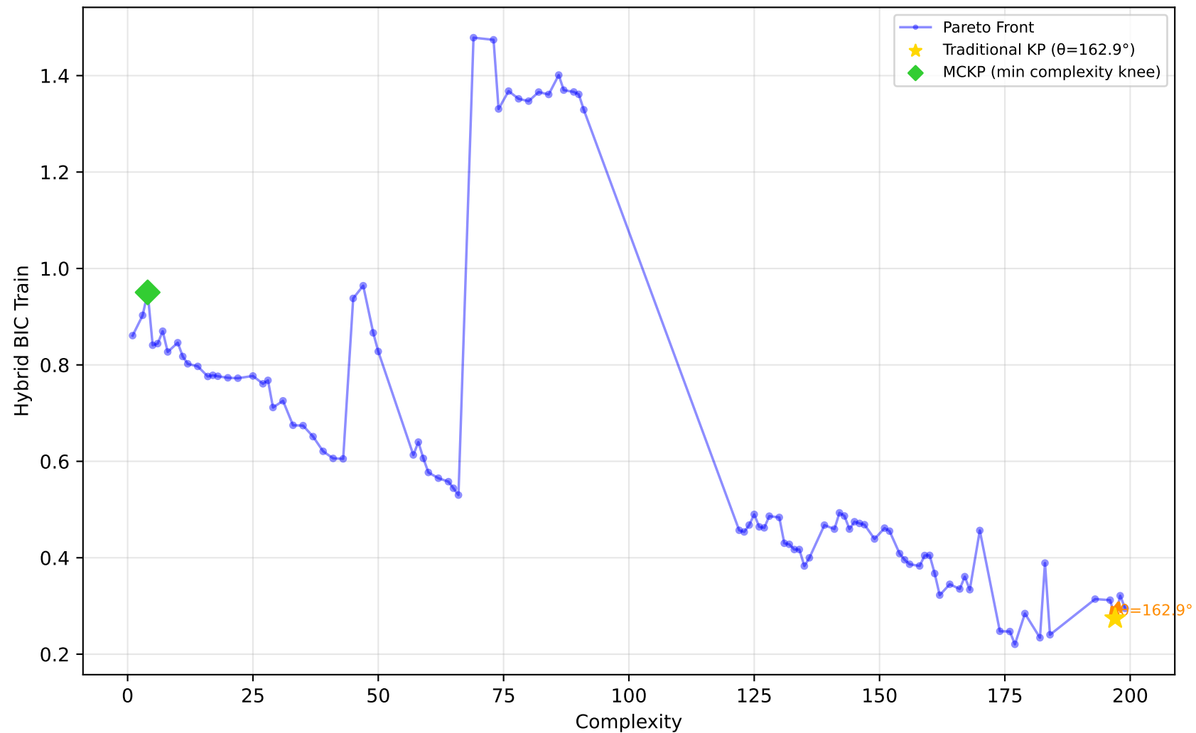
542_pollution - Run 7 - MVP - Hybrid BIC Train \lambda_1=1.00, \lambda_2=0.10, \lambda_3=0.00 | Difficulty: 1.00 | Method: hmr
