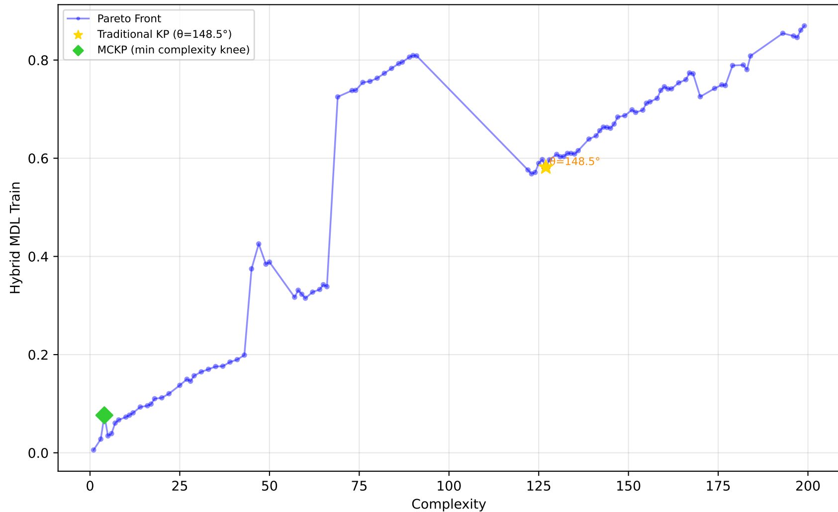
542_pollution - Run 7 - MVP - Hybrid MDL Train \lambda_1=0.40, \lambda_2=0.10, \lambda_3=0.00 | Difficulty: 1.00 | Method: hmr
