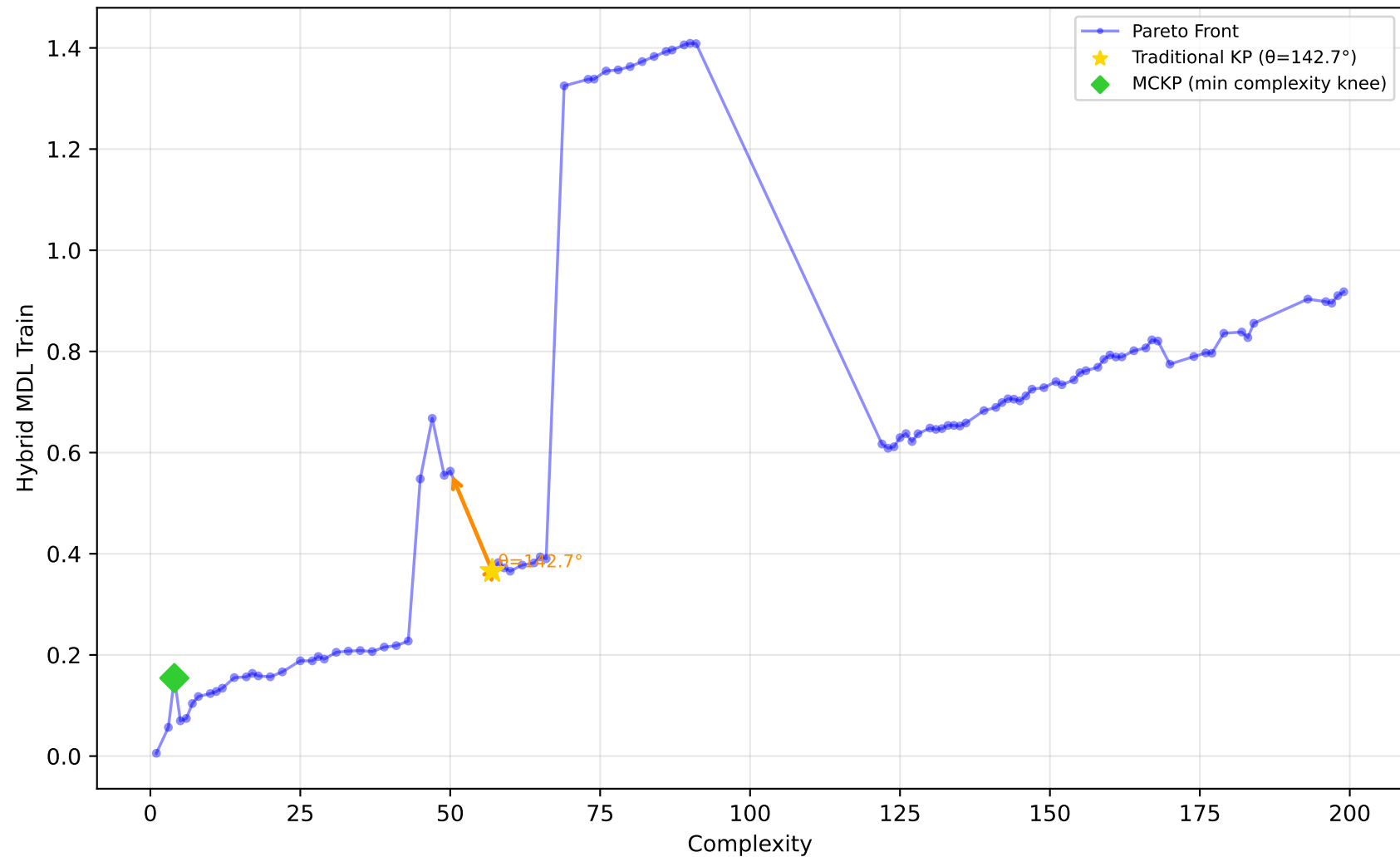
542_pollution - Run 7 - MVP - Hybrid MDL Train \lambda_1=1.00, \lambda_2=0.10, \lambda_3=0.00 | Difficulty: 1.00 | Method: hmr
