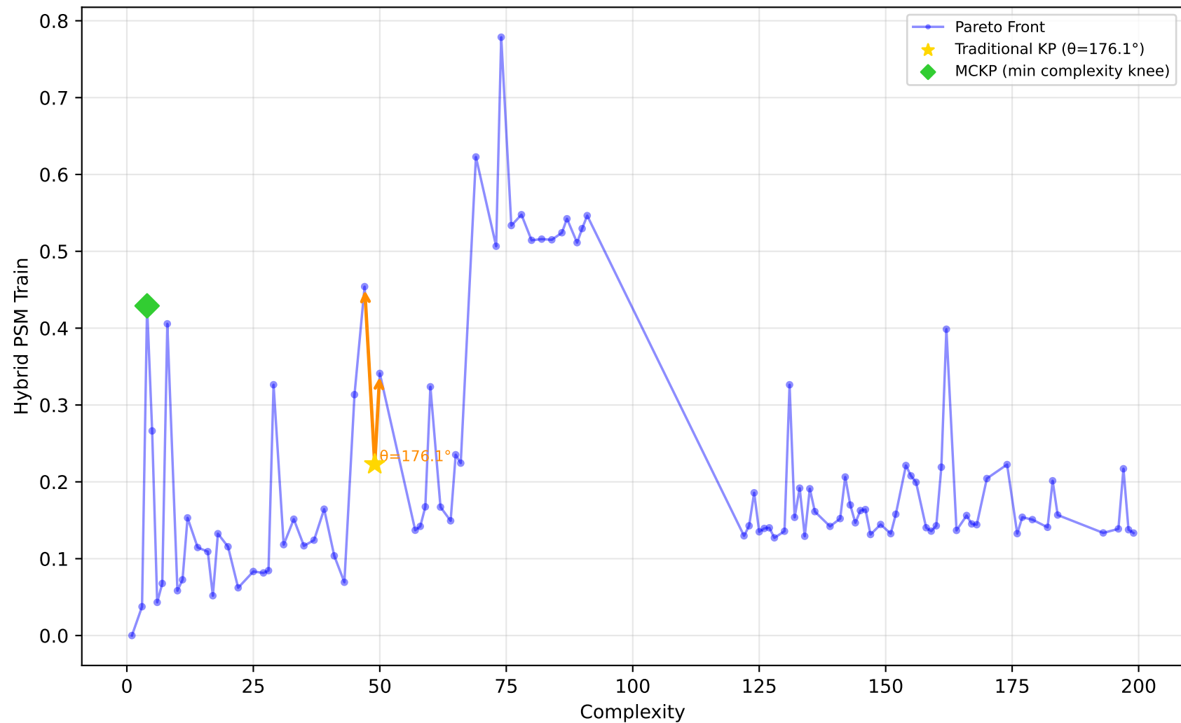
542_pollution - Run 7 - MVP - Hybrid PSM Train \lambda_1=0.40, \lambda_2=0.10, \lambda_3=0.00 | Difficulty: 1.00 | Method: hmr
