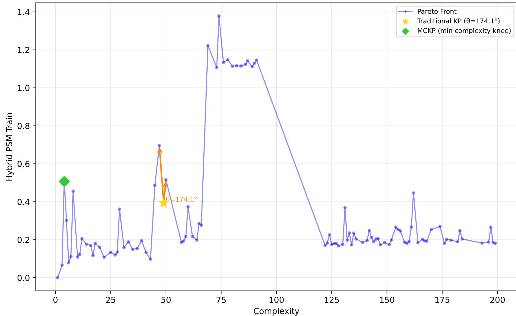
542_pollution - Run 7 - MVP - Hybrid PSM Train \lambda_1=1.00, \lambda_2=0.10, \lambda_3=0.00 | Difficulty: 1.00 | Method: hmr
