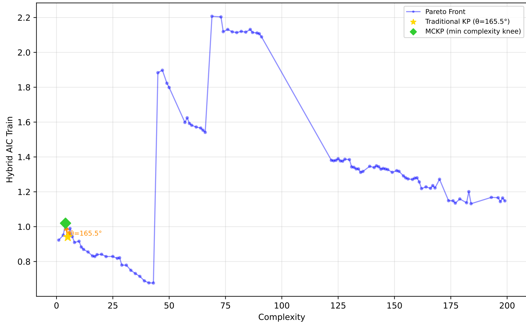
542_pollution - Run 7 - SVP - Hybrid AIC Train \lambda_1=0.70, \lambda_2=1.00, \lambda_3=0.10 | Difficulty: 1.00 | Method: hmr
