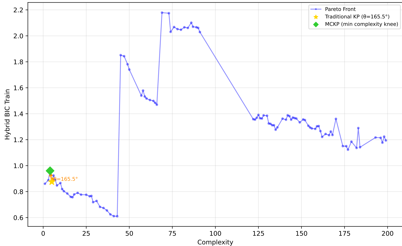
542_pollution - Run 7 - SVP - Hybrid BIC Train \lambda_1=0.70, \lambda_2=1.00, \lambda_3=0.10 | Difficulty: 1.00 | Method: hmr
