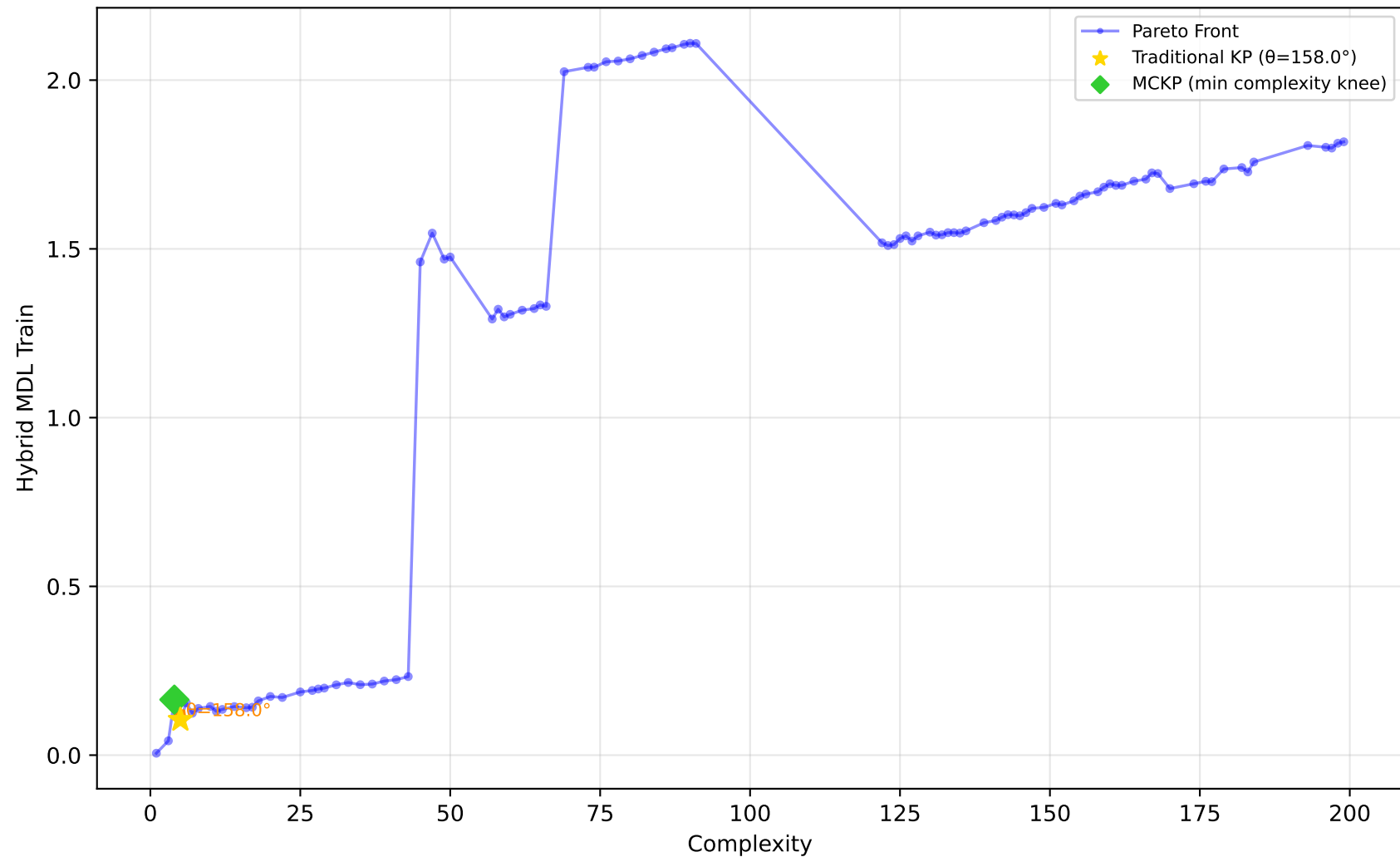
542_pollution - Run 7 - SVP - Hybrid MDL Train \lambda_1=0.70, \lambda_2=1.00, \lambda_3=0.10 | Difficulty: 1.00 | Method: hmr
