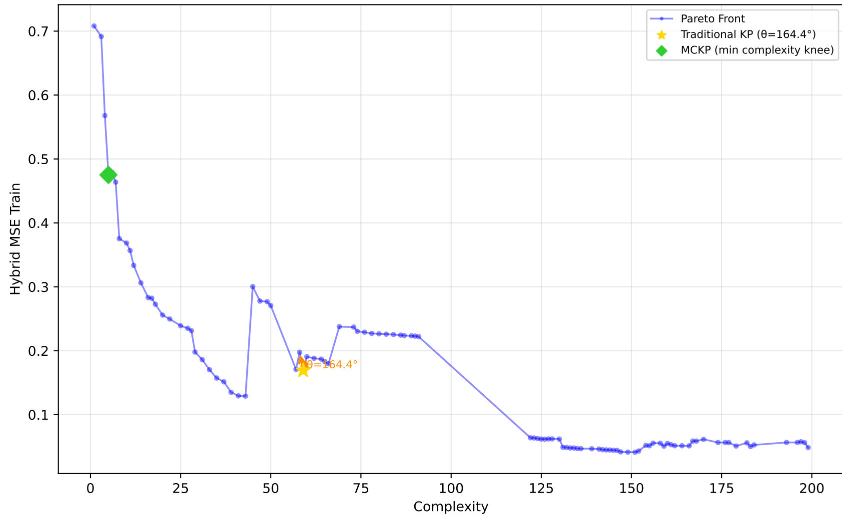
542_pollution - Run 7 - SVP - Hybrid MSE Train \lambda_1=0.00, \lambda_2=0.00, \lambda_3=0.20 | Difficulty: 1.00 | Method: hmr
