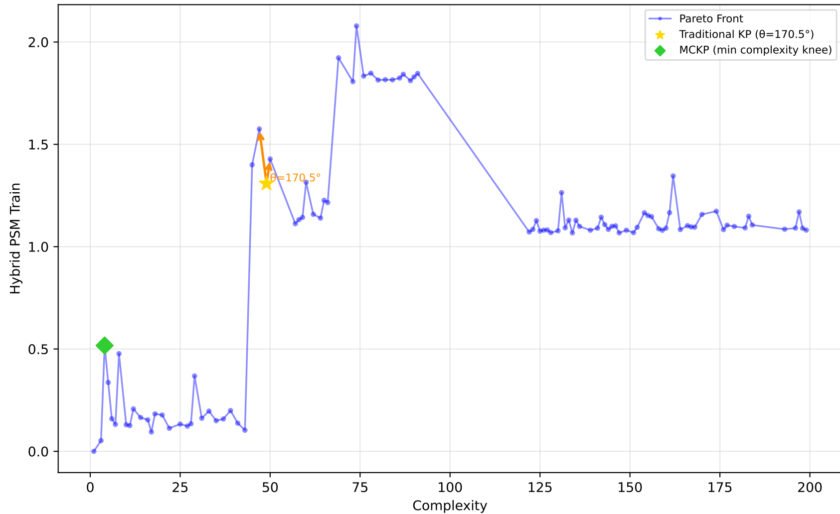
542_pollution - Run 7 - SVP - Hybrid PSM Train \lambda_1=0.70, \lambda_2=1.00, \lambda_3=0.10 | Difficulty: 1.00 | Method: hmr
