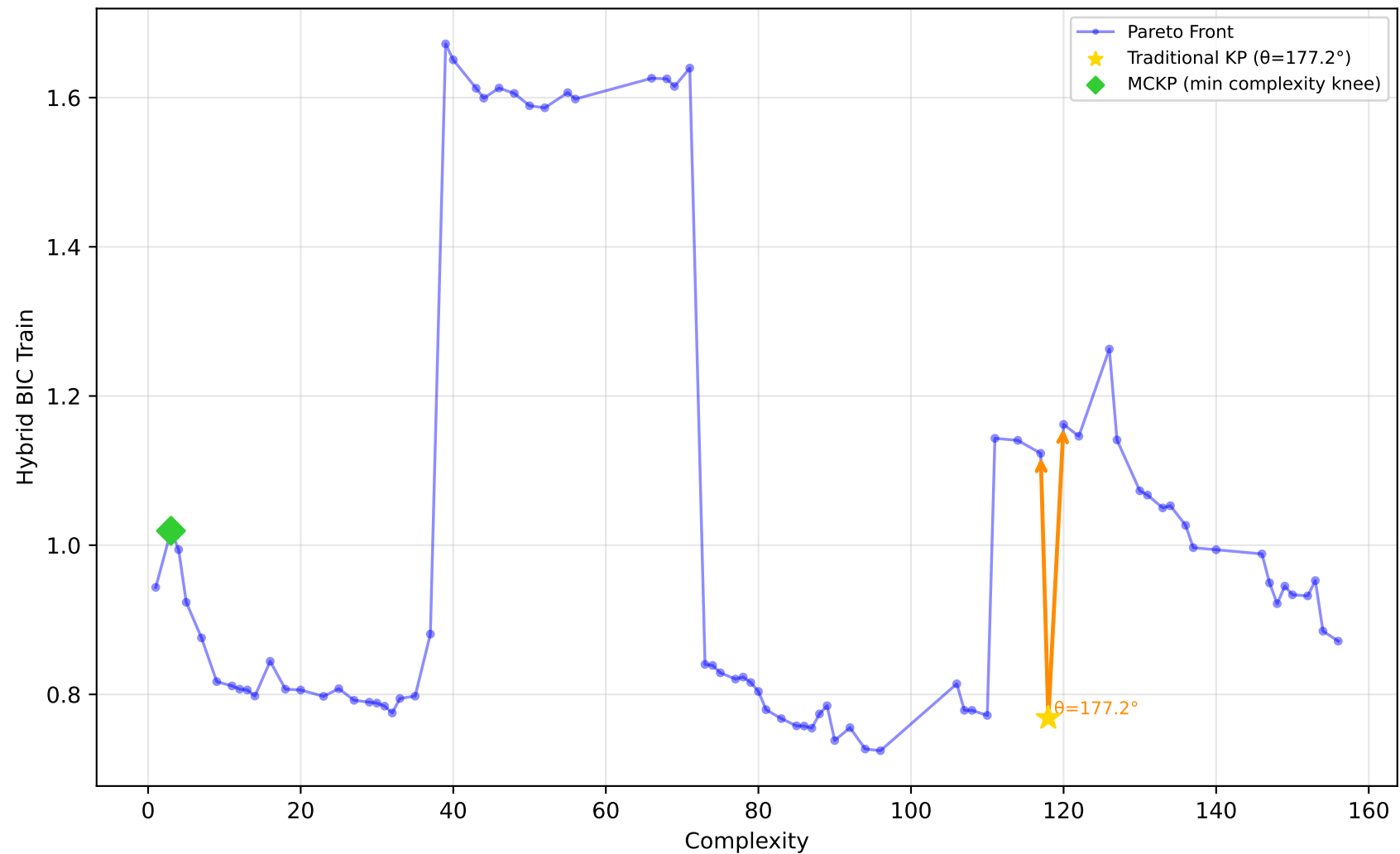
542_pollution - Run 8 - MVP - Hybrid BIC Train \lambda_1=1.00, \lambda_2=0.10, \lambda_3=0.00 | Difficulty: 0.23 | Method: mckp
