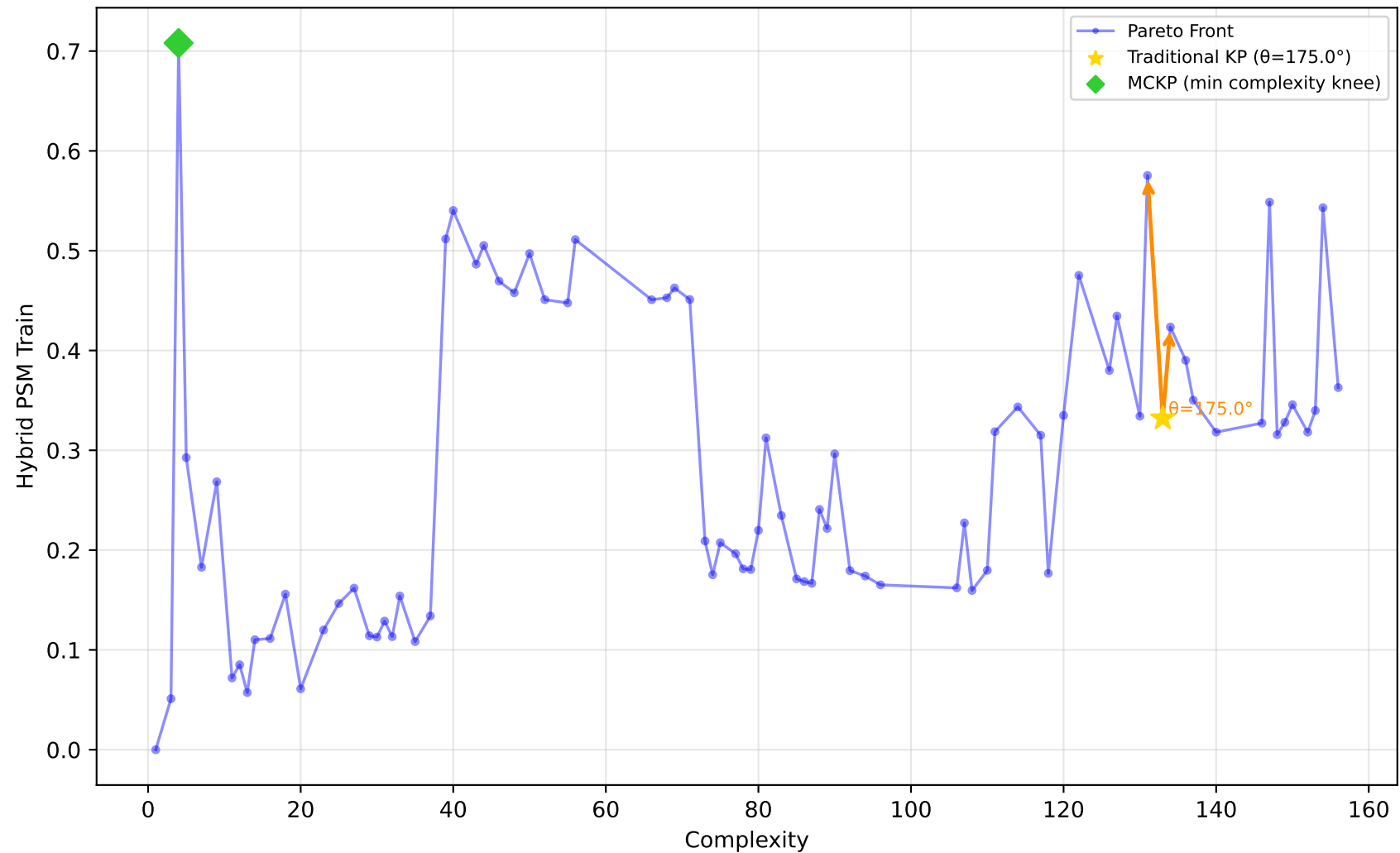
542_pollution - Run 8 - MVP - Hybrid PSM Train \lambda_1=0.40, \lambda_2=0.10, \lambda_3=0.00 | Difficulty: 0.23 | Method: mckp
