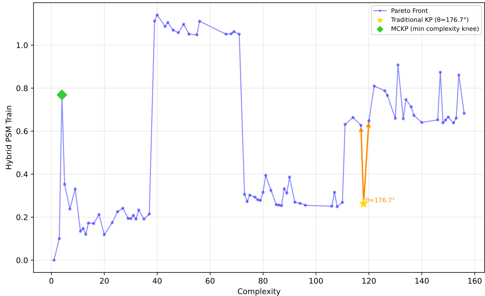
542_pollution - Run 8 - MVP - Hybrid PSM Train \lambda_1=1.00, \lambda_2=0.10, \lambda_3=0.00 | Difficulty: 0.23 | Method: mckp
