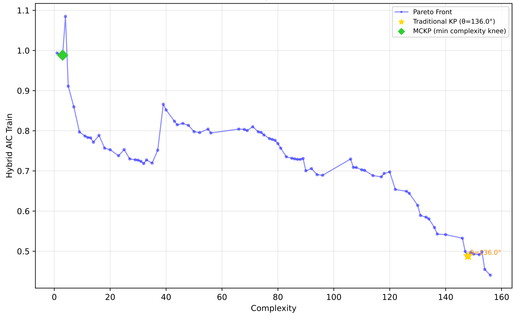
542_pollution - Run 8 - SVP - Hybrid AIC Train \lambda_1=0.00, \lambda_2=0.00, \lambda_3=0.20 | Difficulty: 0.23 | Method: mckp
