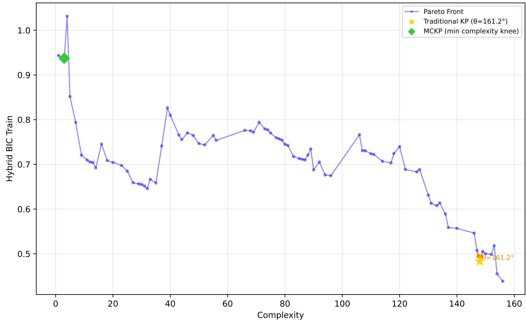
542_pollution - Run 8 - SVP - Hybrid BIC Train \lambda_1=0.00, \lambda_2=0.00, \lambda_3=0.20 | Difficulty: 0.23 | Method: mckp
