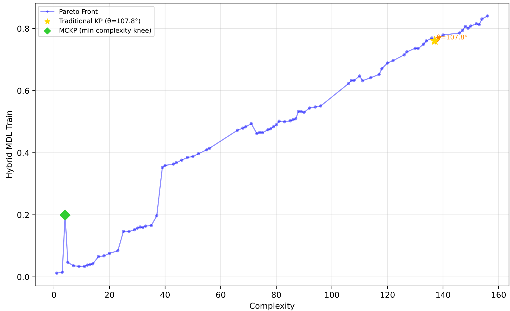
542_pollution - Run 8 - SVP - Hybrid MDL Train \lambda_1=0.00, \lambda_2=0.00, \lambda_3=0.20 | Difficulty: 0.23 | Method: mckp
