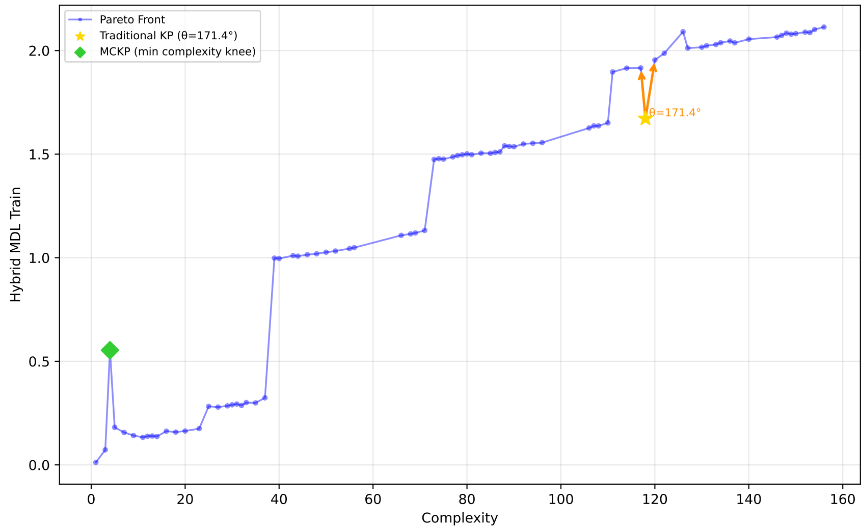
542_pollution - Run 8 - SVP - Hybrid MDL Train \lambda_1=0.70, \lambda_2=1.00, \lambda_3=0.10 | Difficulty: 0.23 | Method: mckp
