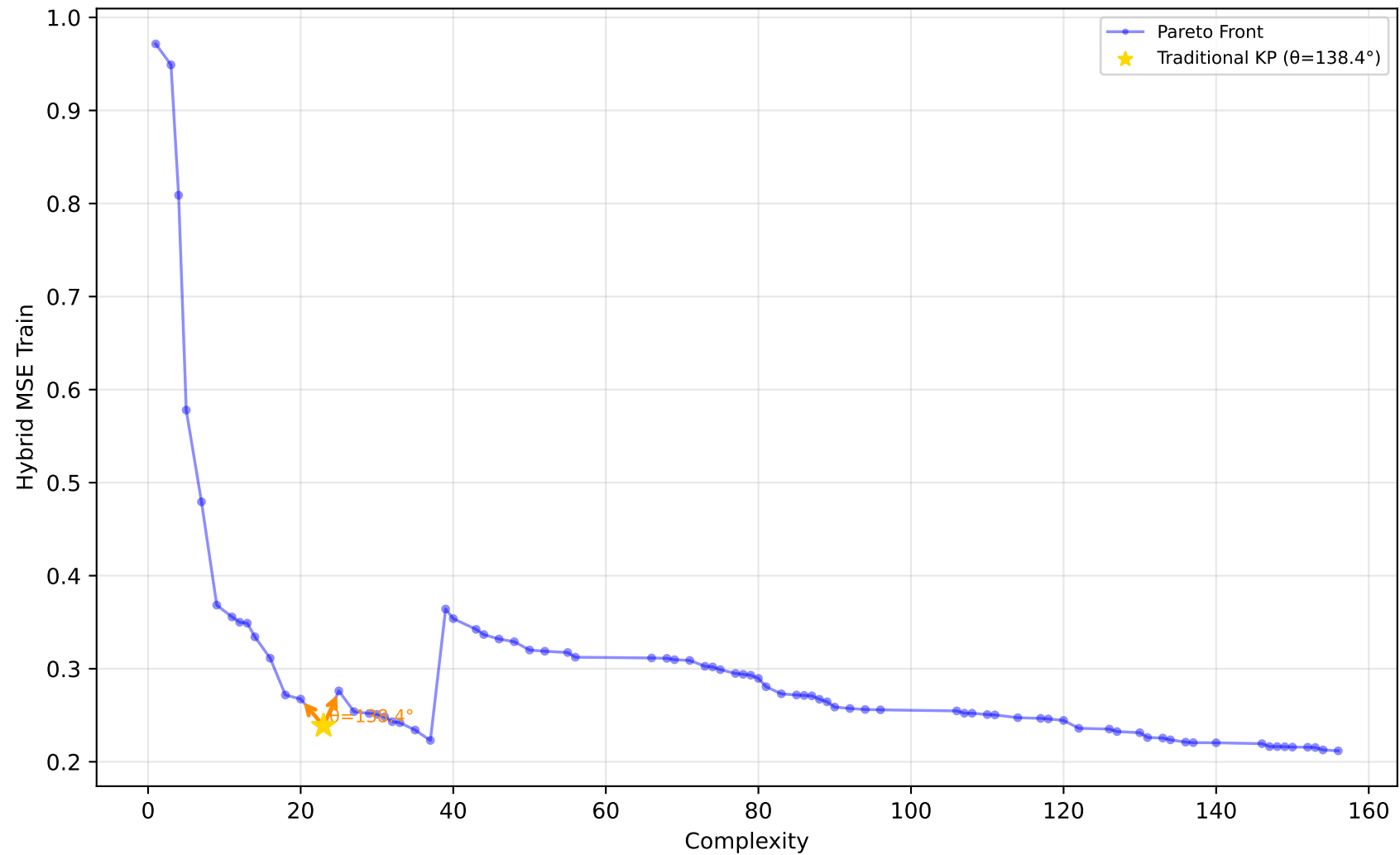
542_pollution - Run 8 - SVP - Hybrid MSE Train \lambda_1=0.00, \lambda_2=0.00, \lambda_3=0.20 | Difficulty: 0.23 | Method: mckp
