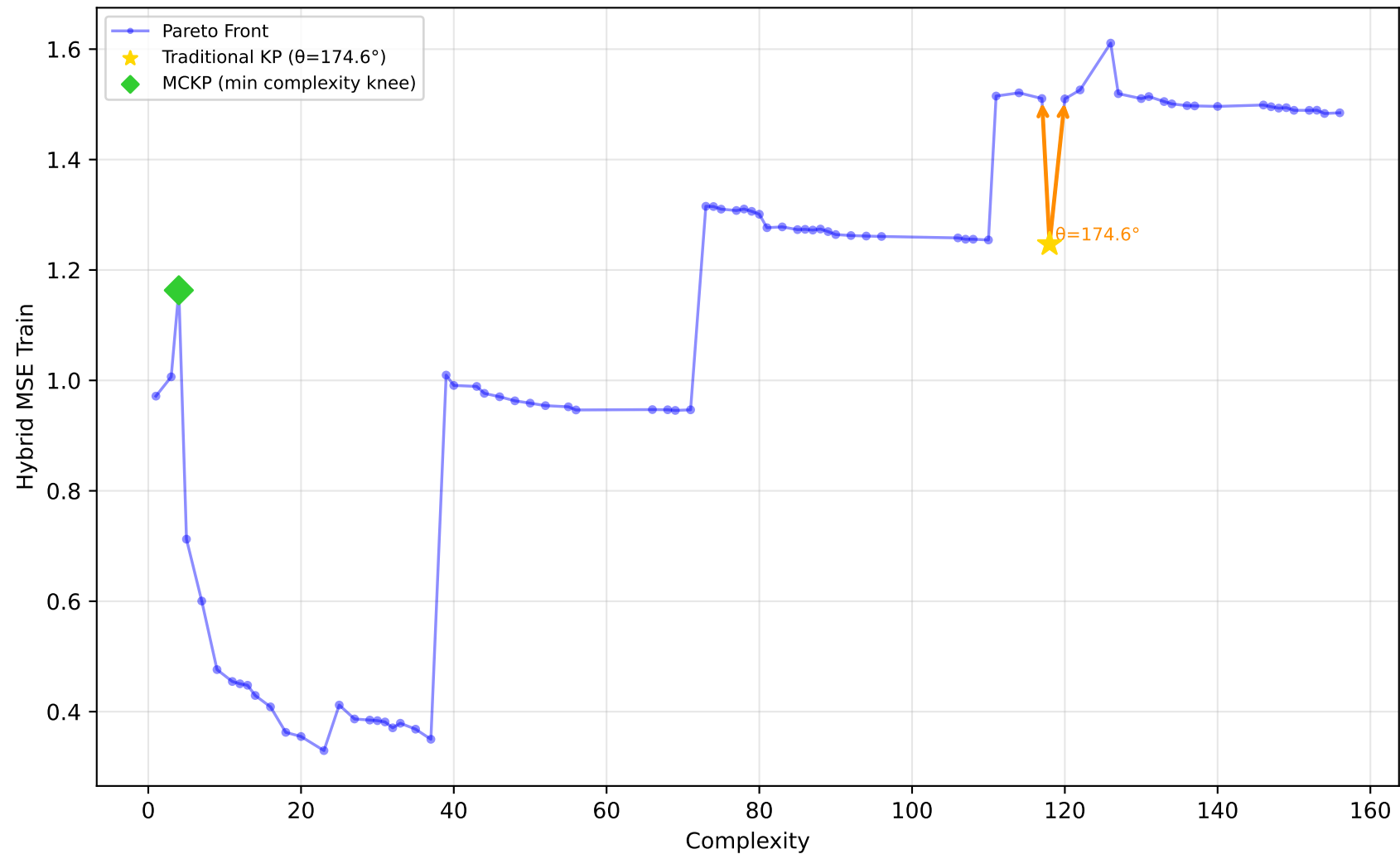
542_pollution - Run 8 - SVP - Hybrid MSE Train \lambda_1=0.70, \lambda_2=1.00, \lambda_3=0.10 | Difficulty: 0.23 | Method: mckp
