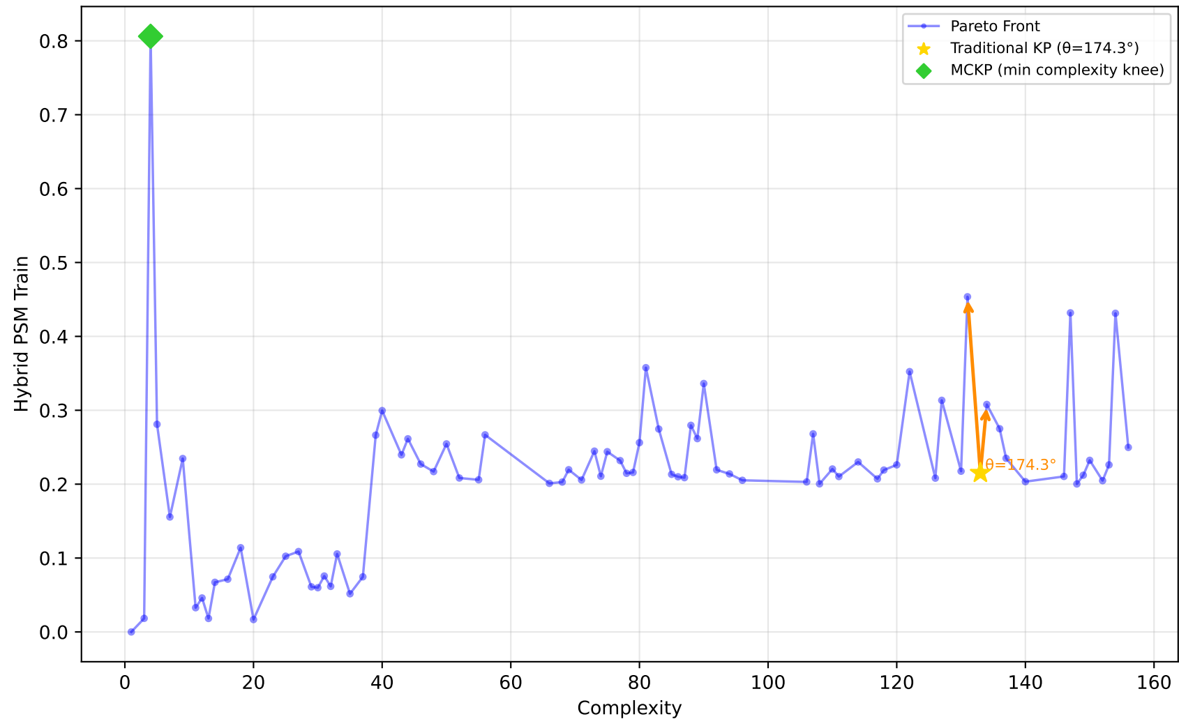
542_pollution - Run 8 - SVP - Hybrid PSM Train \lambda_1=0.00, \lambda_2=0.00, \lambda_3=0.20 | Difficulty: 0.23 | Method: mckp
