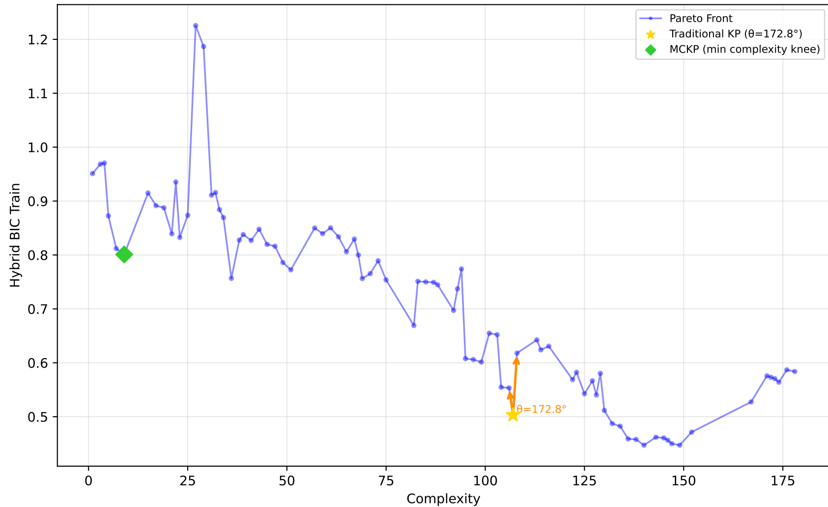
542_pollution - Run 9 - MVP - Hybrid BIC Train \lambda_1=0.40, \lambda_2=0.10, \lambda_3=0.00 | Difficulty: 0.56 | Method: mckp
