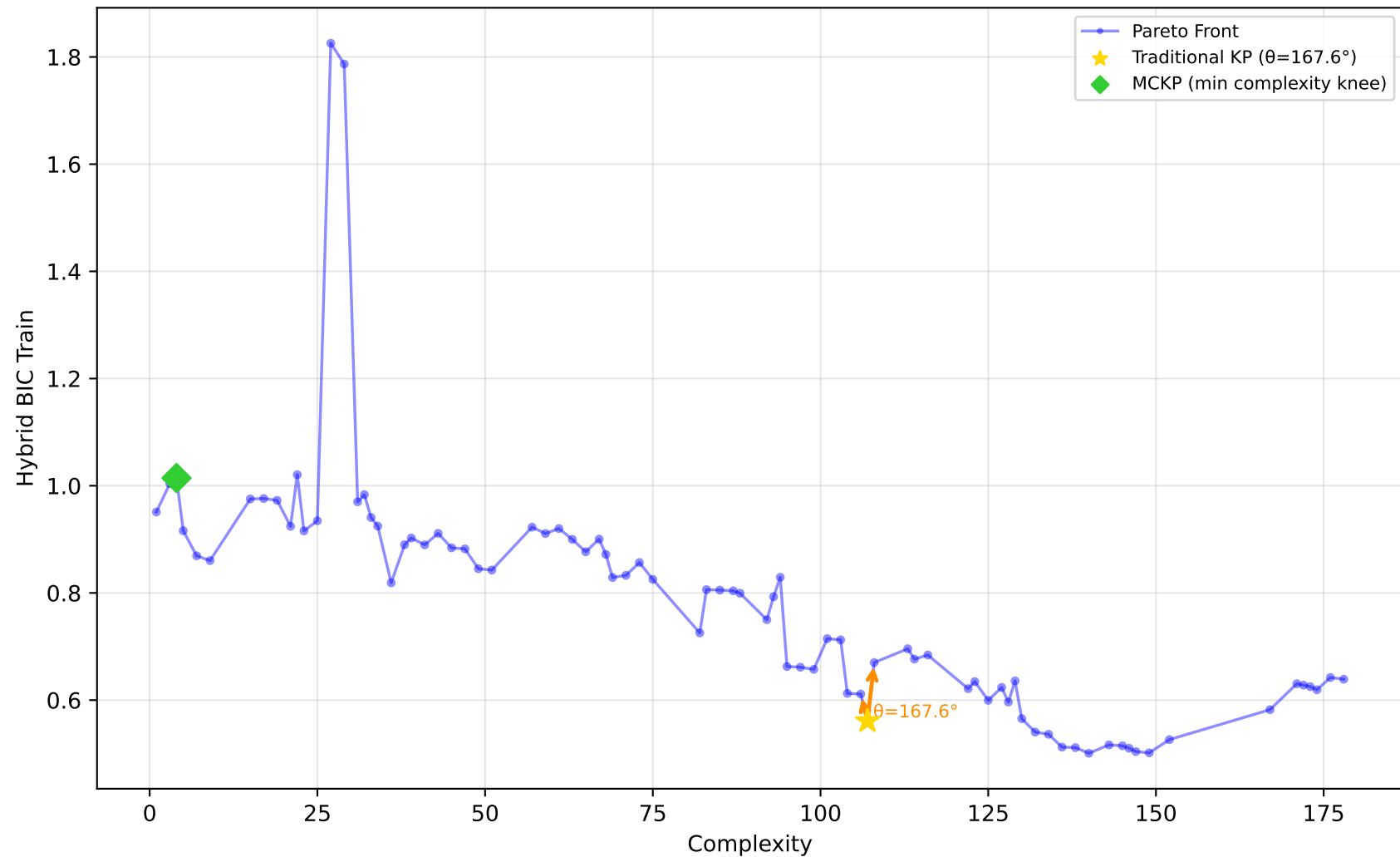
542_pollution - Run 9 - MVP - Hybrid BIC Train \lambda_1=1.00, \lambda_2=0.10, \lambda_3=0.00 | Difficulty: 0.56 | Method: mckp
