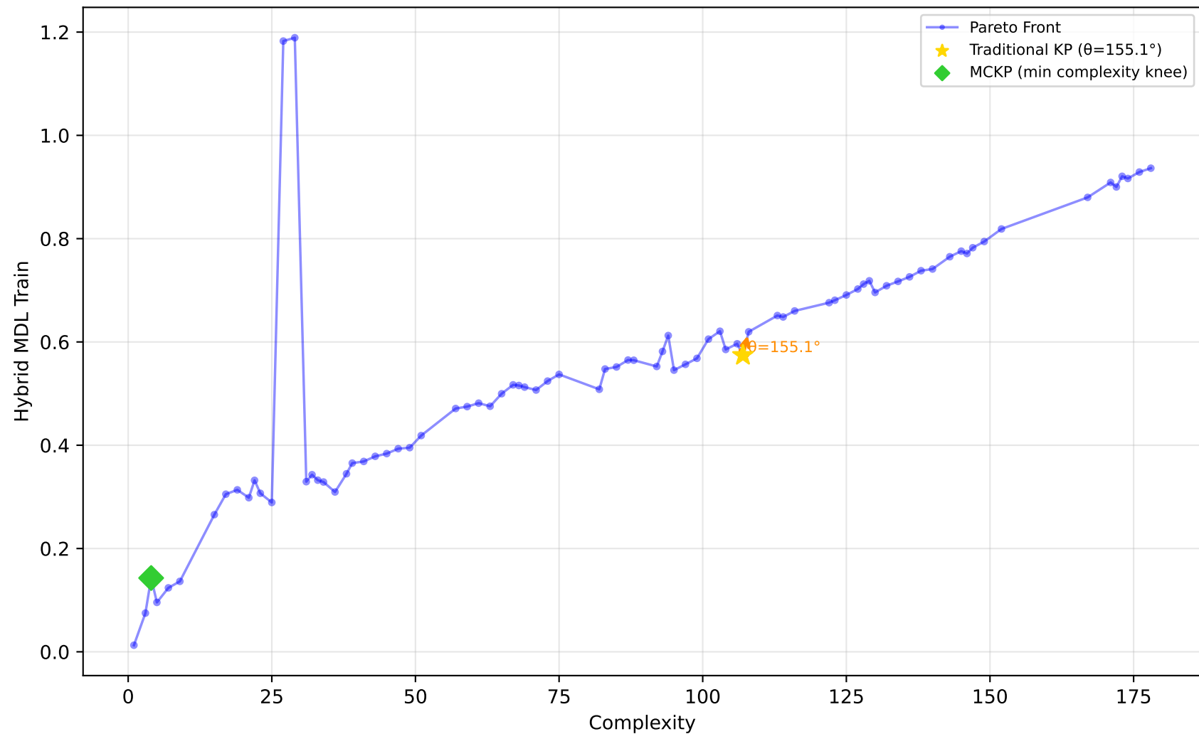
542_pollution - Run 9 - MVP - Hybrid MDL Train \lambda_1=1.00, \lambda_2=0.10, \lambda_3=0.00 | Difficulty: 0.56 | Method: mckp
