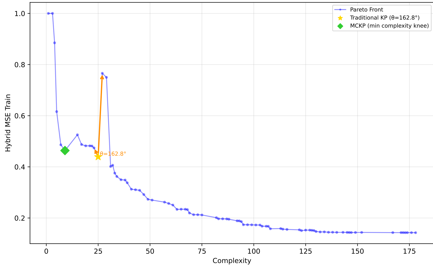
542_pollution - Run 9 - MVP - Hybrid MSE Train \lambda_1=0.40, \lambda_2=0.10, \lambda_3=0.00 | Difficulty: 0.56 | Method: mckp
