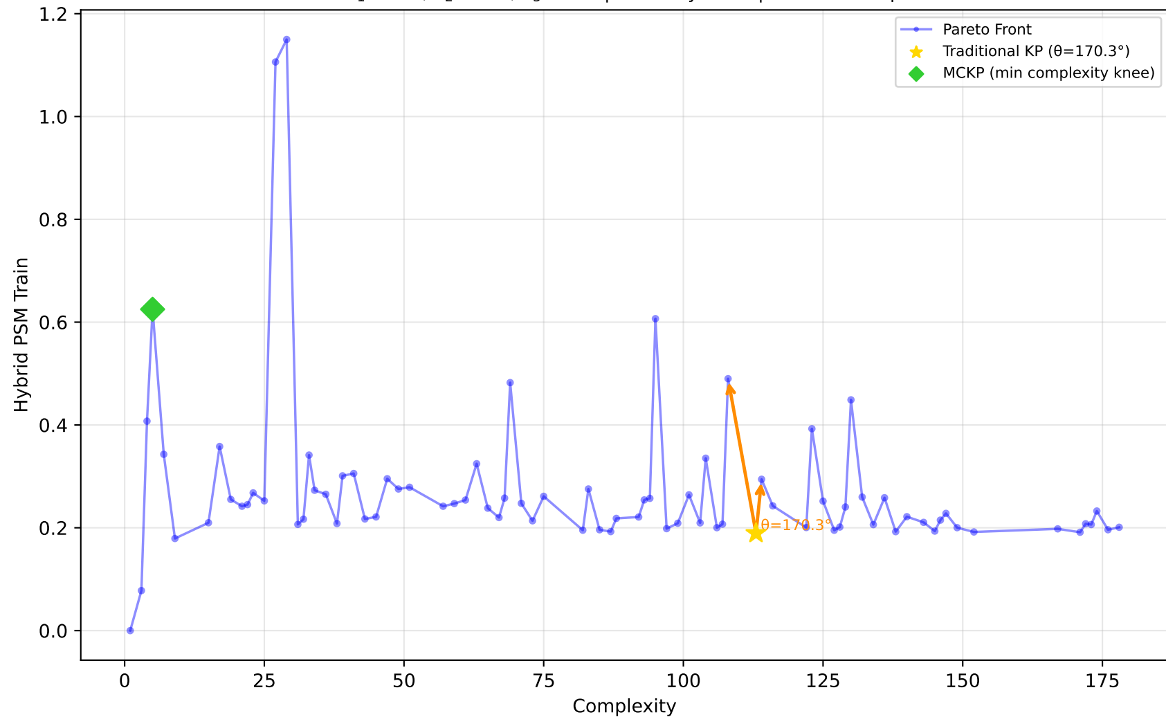
542_pollution - Run 9 - MVP - Hybrid PSM Train \lambda_1=1.00, \lambda_2=0.10, \lambda_3=0.00 | Difficulty: 0.56 | Method: mckp
