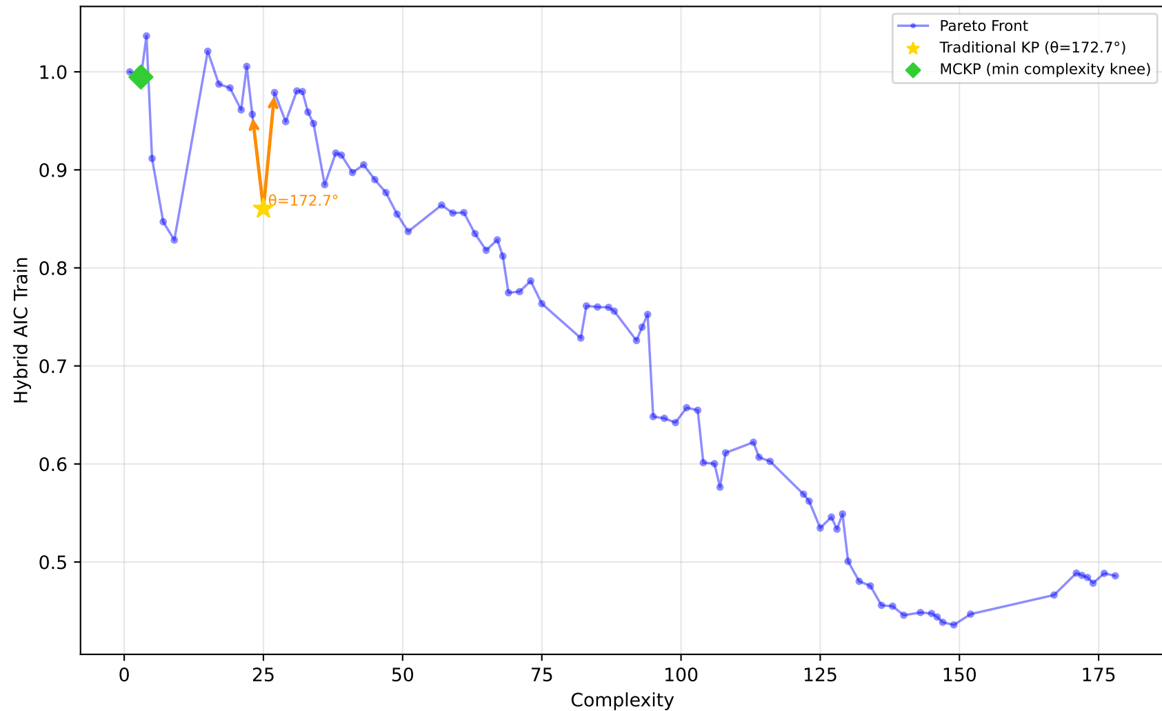
542_pollution - Run 9 - SVP - Hybrid AIC Train \lambda_1=0.00, \lambda_2=0.00, \lambda_3=0.20 | Difficulty: 0.56 | Method: mckp
