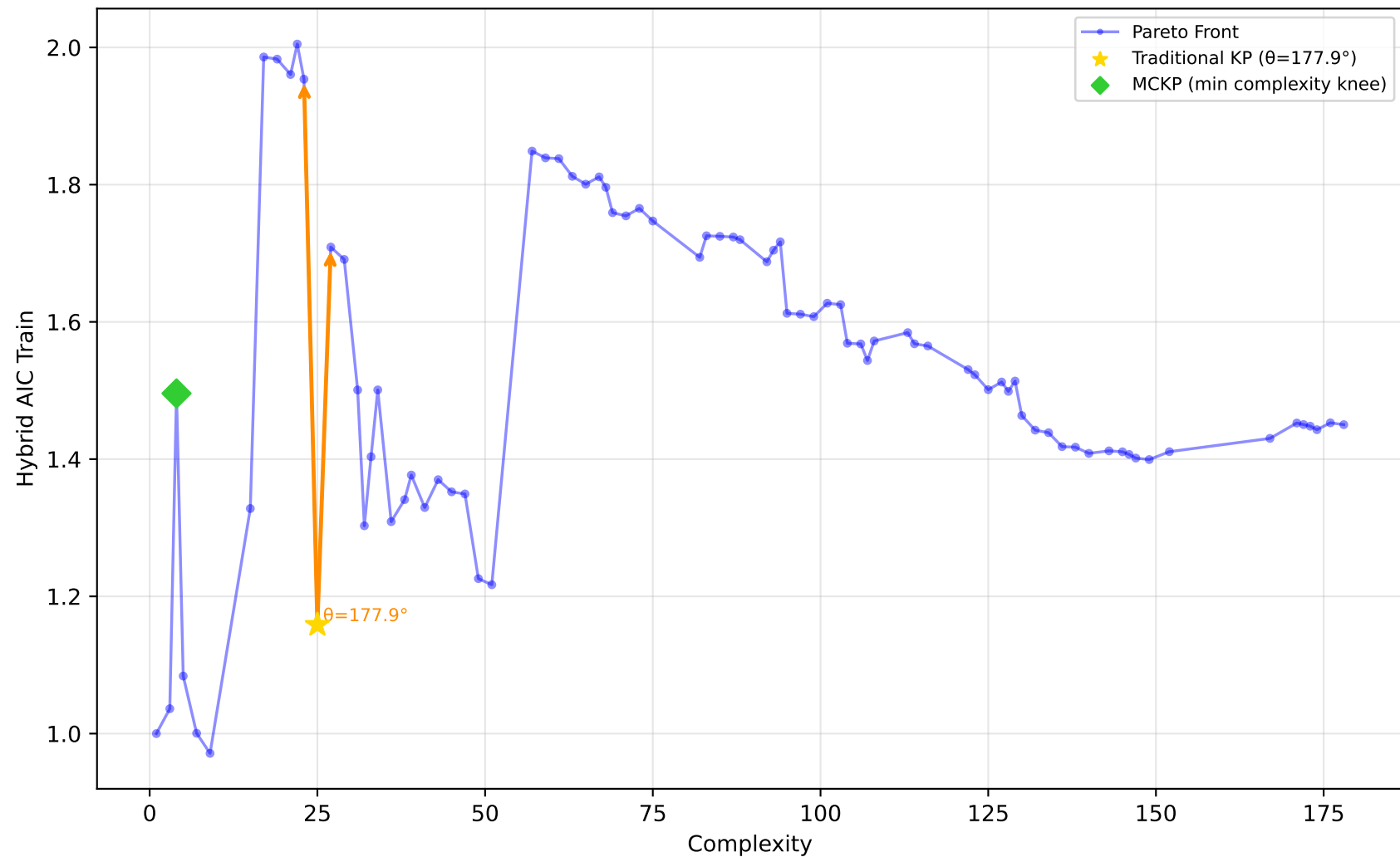
542_pollution - Run 9 - SVP - Hybrid AIC Train \lambda_1=0.70 , \lambda_2=1.00 , \lambda_3=0.10 | Difficulty: 0.56 | Method: mckp
