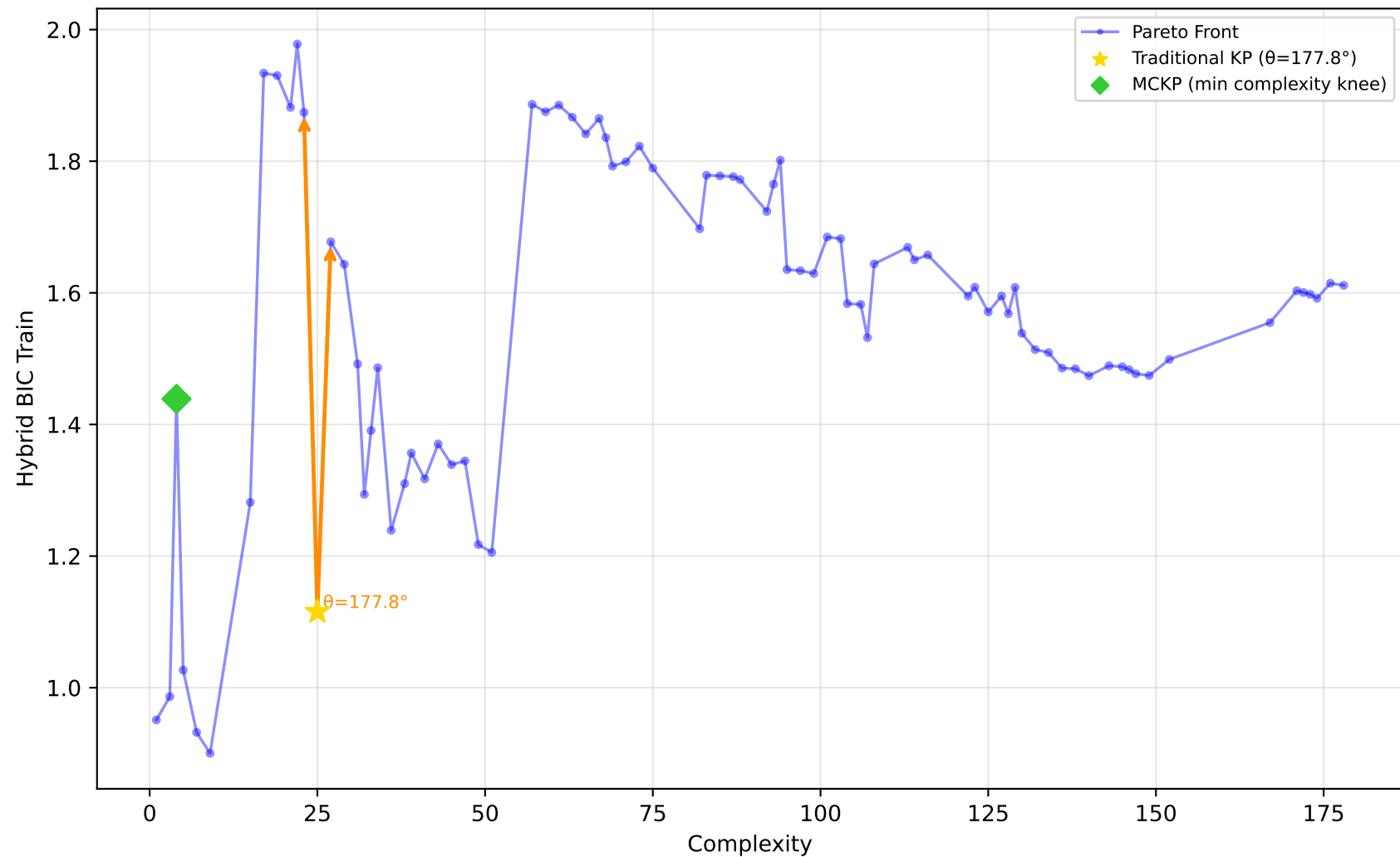
542_pollution - Run 9 - SVP - Hybrid BIC Train \lambda_1=0.70 , \lambda_2=1.00 , \lambda_3=0.10 | Difficulty: 0.56 | Method: mckp
