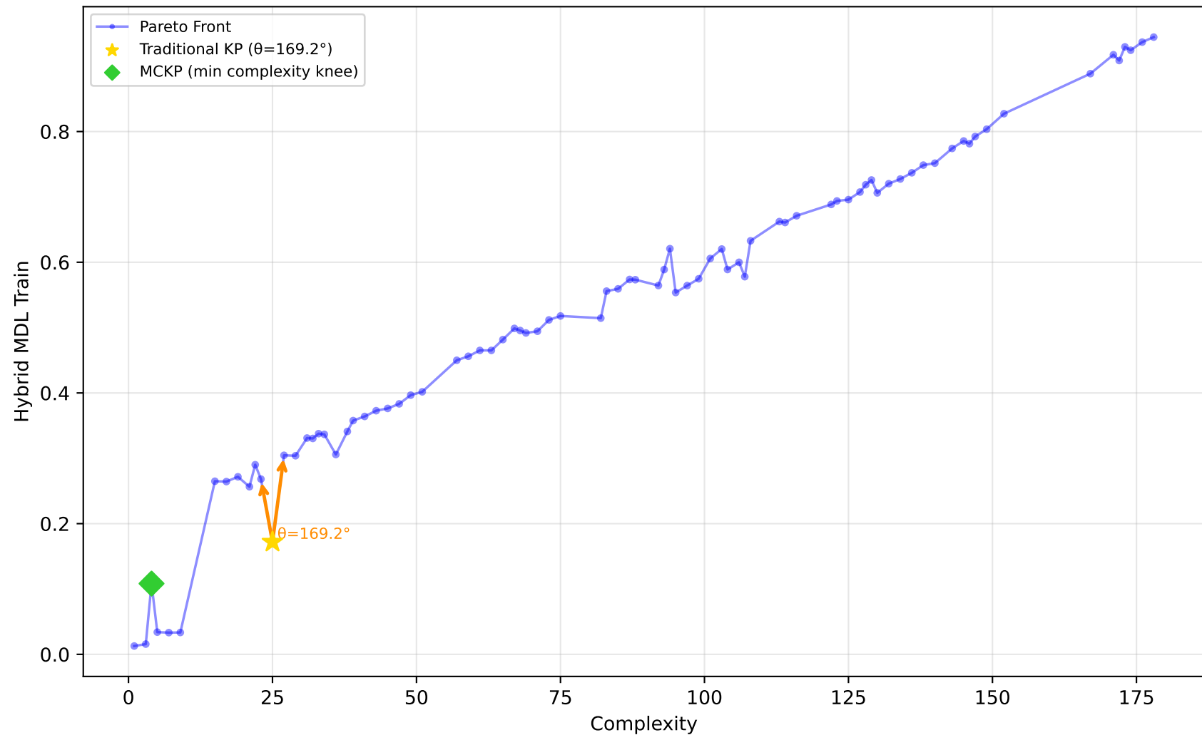
542_pollution - Run 9 - SVP - Hybrid MDL Train \lambda_1=0.00, \lambda_2=0.00, \lambda_3=0.20 | Difficulty: 0.56 | Method: mckp
