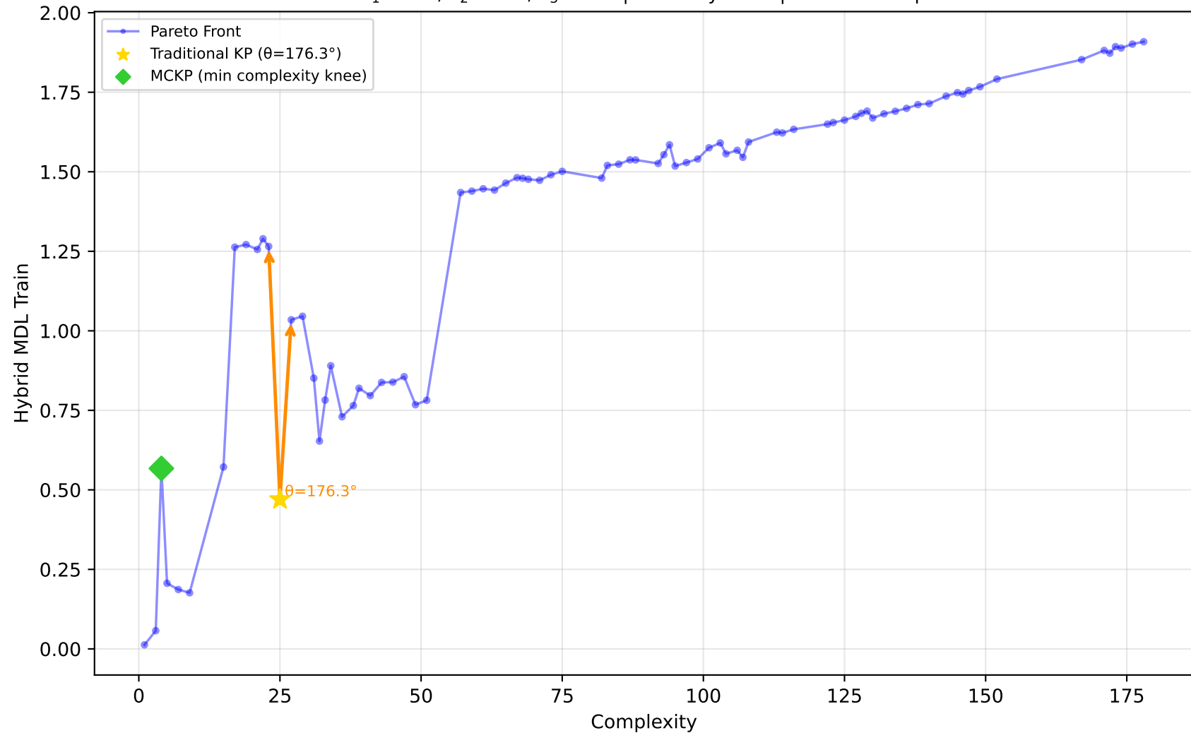
542_pollution - Run 9 - SVP - Hybrid MDL Train \lambda_1=0.70, \lambda_2=1.00, \lambda_3=0.10 | Difficulty: 0.56 | Method: mckp
