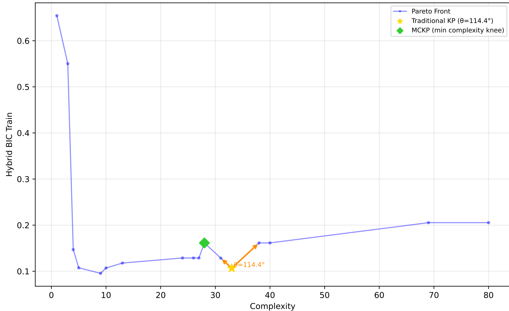
523_analcatdata_neavote - Run 10 - MVP - Hybrid BIC Train \lambda_1=0.00, \lambda_2=0.10, \lambda_3=0.00 | Difficulty: 1.00 | Method: hmr
