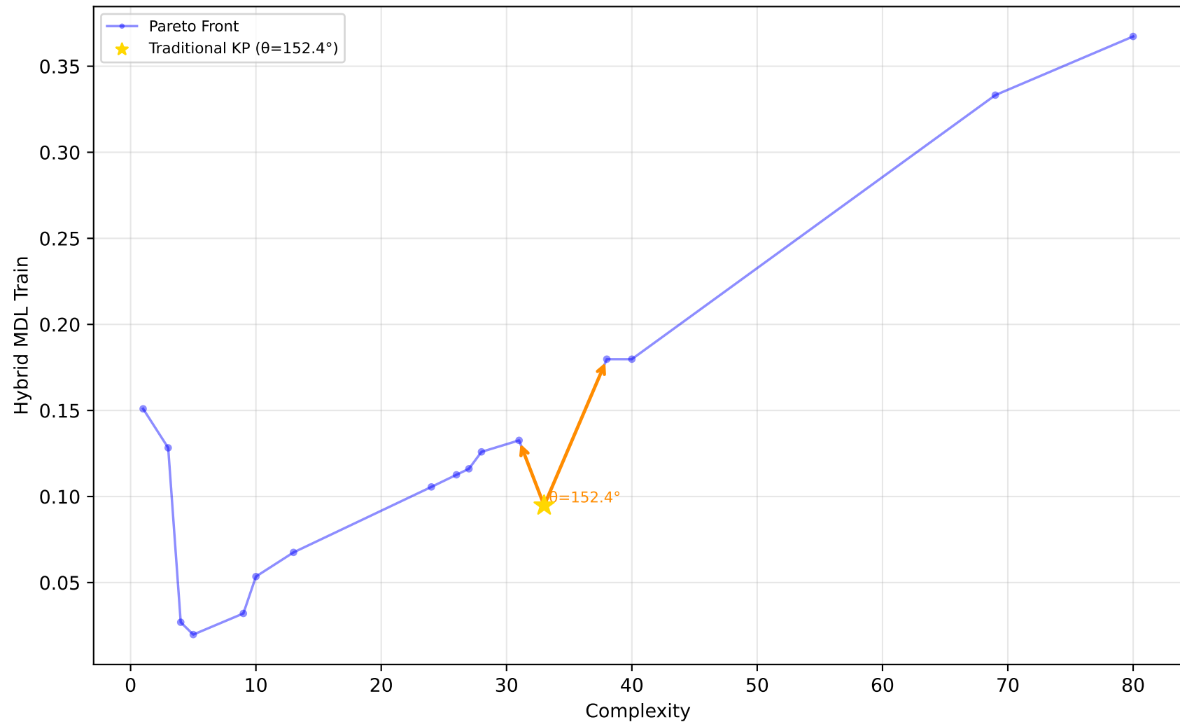
523_analcatdata_neavote - Run 10 - MVP - Hybrid MDL Train \lambda_1=0.00, \lambda_2=0.10, \lambda_3=0.00 | Difficulty: 1.00 | Method: hmr
