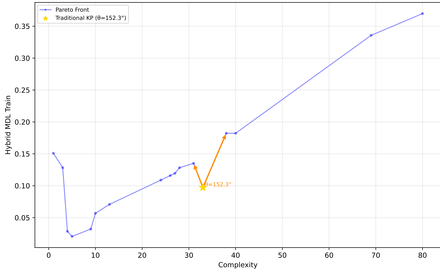
523_analcatdata_neavote - Run 10 - MVP - Hybrid MDL Train \lambda_1=0.00, \lambda_2=0.40, \lambda_3=0.00 | Difficulty: 1.00 | Method: hmr
